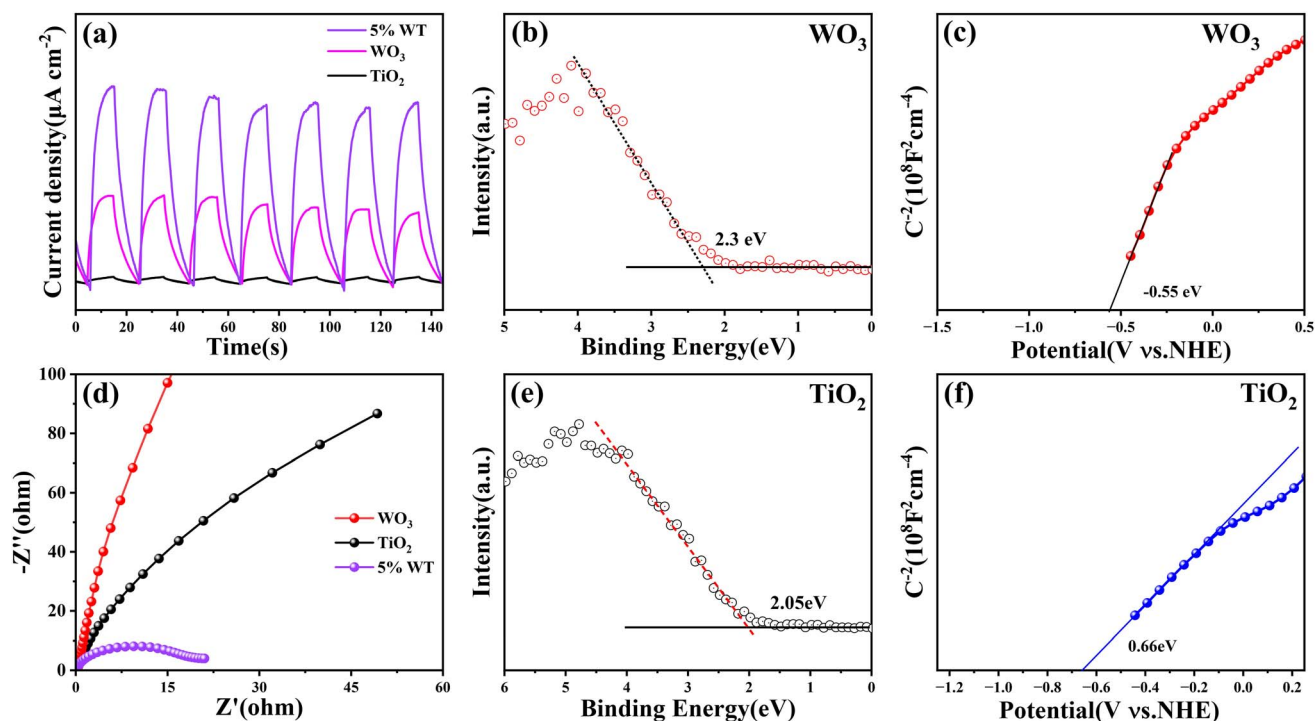
Fig. 12 (a) Transient photocurrent response of TiO 2 , WO 3 and 5% WT; (b) XPS VB spectrum of WO 3 ; (c) Mott-Schottky plot of WO 3 ; (d) Nyquist plot of TiO 2 , WO 3 and 5% WT; (e) XPS VB spectrum of TiO 2 ; (f) Mott-Schottky plot of TiO 2 .
