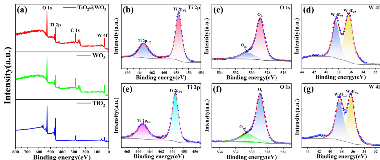
Fig. 4 (a) Full scan XPS spectra of \text{TiO}_2 , \text{WO}_3 , and \text{WO}_3/\text{TiO}_2 ; (b) Ti 2p XPS spectrum of \text{TiO}_2 ; (c) O 1s XPS spectrum of \text{WO}_3 ; (d) W 4f XPS spectrum of \text{WO}_3 ; (e) Ti 2p XPS spectrum of \text{WO}_3/\text{TiO}_2 ; (f) O 1s XPS spectrum of \text{WO}_3/\text{TiO}_2 ; (g) W 4f XPS spectrum of \text{WO}_3/\text{TiO}_2 .
