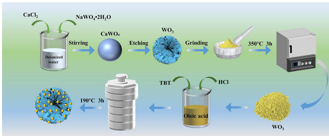
Fig. 1 Schematic illustration of the synthesis process of \text{WO}_3@\text{TiO}_2 heterojunction composite material.
