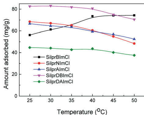
Fig. 7 Effect of temperature on the adsorption of 2,4-DNP onto the five adsorbents.
