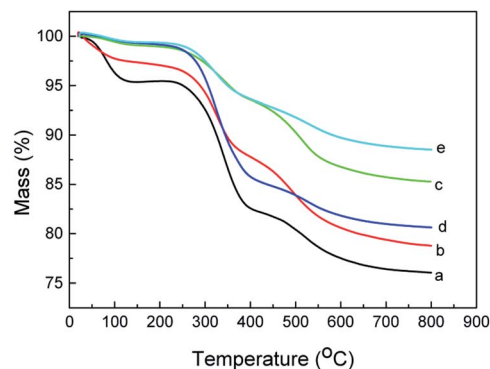
Fig. 4 Thermogravimetric curves of SilprBImCl (a), SilprNImCl (b), SilprAlmCl (c), SilprDBImCl (d) and SilprDAImCl (e).
