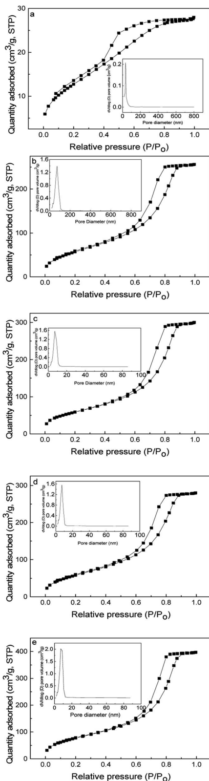
Fig. 3 N_2 adsorption-desorption isotherms and pore size distributions of SilprBImCl (a), SilprNImCl (b), SilprAlmCl (c), SilprDBImCl (d) and SilprDAImCl (e).
