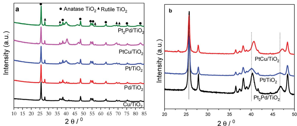
Fig. 2 PXRD patterns of TiO 2 nanofiber photocatalysts (a) deposited with various co-catalysts. (b) PXRD patterns of 2%Pt/TiO 2 , 2%Pt 2 Pd/TiO 2 , and 2%PtCu/TiO 2 nanofiber photocatalysts in the region 20° ≤ 2θ ≤ 50°.
