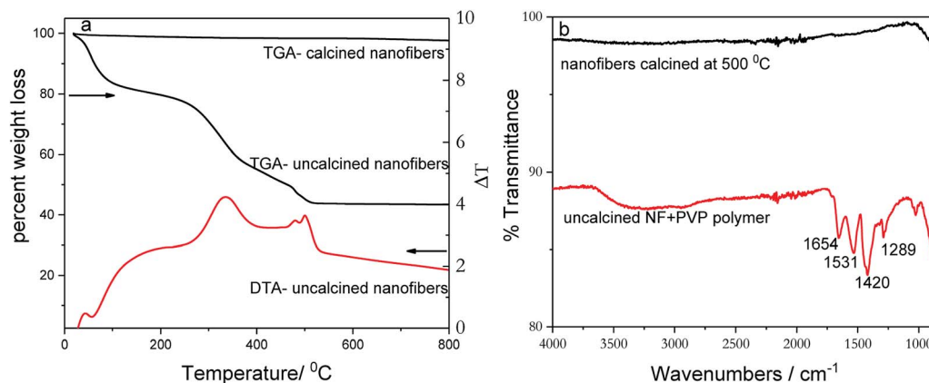
Fig. 1 TGA and DTA plots of (a) calcined and uncalcined TiO 2 nanofibers acquired by heating in air. (b) FTIR spectra of calcined and uncalcined TiO 2 nanofibers.
