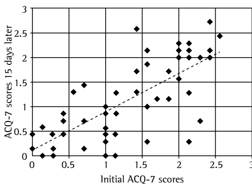
Figure 1 – Correlation between the Asthma Control Questionnaire 7 (ACQ-7) scores obtained in the initial visit and those obtained 15 days later in the 52 patients studied. r = 0.73 ; 95% CI: 0.58-0.83; p < 0.0001 .
