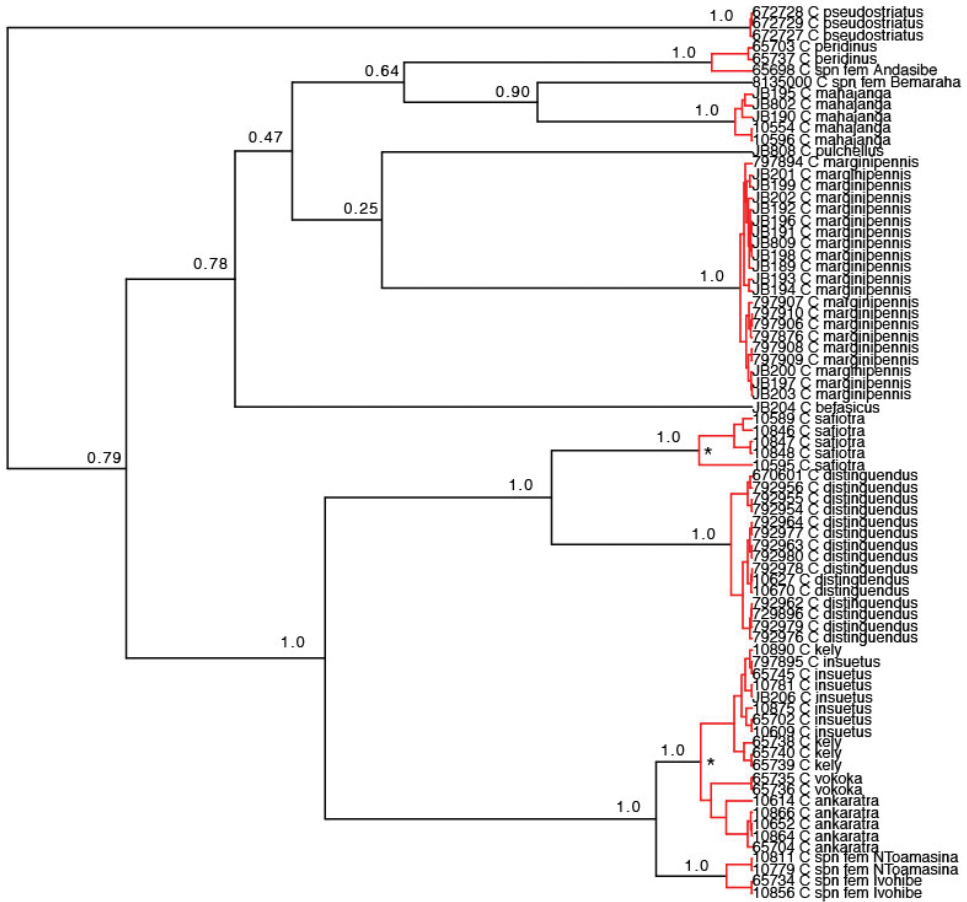
Figure 3. Result of the single-locus GMYC species delimitation using an ultrametric CO1 genetree from BEAST. Black branches indicate interspecific divergences, red branches represent intraspecific coalescence events. Values above interspecific nodes indicate posterior probability from the Beast analysis under a strict clock model. The * indicates two nodes of further splitting from the GMYC analysis that is within the confidence interval of 2Log likelihood units from the optimal solution.
