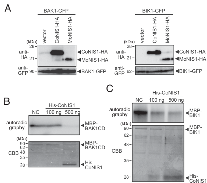
Fig. 5. NIS1 inhibits the kinase activity of both BAK1 and BIK1. (A) Effects of NIS1 homologs (CoNIS1 and MoNIS1) on protein stability of BAK1 (Left) and BIK1 (Right). CoNIS1-HA or MoNIS1-HA were transiently coexpressed with BAK1-GFP or BIK1-GFP in Nb. A. tumefaciens harboring the empty plasmid pBICP35 was infiltrated (vector) as a control for the expression of CoNIS1-HA and MoNIS1-HA. Protein extracts were analyzed by immunoblotting with anti-HA and anti-GFP antibodies. (B) NIS1 inhibits autophosphorylation of BAK1. Purified MBP-fused BAK1 cytoplasmic domain (MBP-BAK1CD) were incubated with His-tagged CoNIS1 proteins purified from the culture medium of BY-2 cells secreting CoNIS1 (CoNIS1, 500 ng). We incubated MBP-fused kinase proteins with the equivalent fraction purified from the culture medium of BY-2 cells that do not secrete CoNIS1 as a negative control (NC). The His-tagged CoNIS1 protein fraction was also diluted fivefold with kinase reaction buffer and used for the assay (CoNIS1, 100 ng). In vitro kinase assay using [ \gamma - ^{32} P] ATP was performed and autophosphorylation was visualized by autoradiography. CBB was used as a loading control. Similar results were obtained from one additional experiment. (C) NIS1 inhibits autophosphorylation of BIK1. Purified MBP-fused BIK1 (MBP-BIK1) were subjected to the analysis described in B. Similar results were obtained from three additional experiments.
