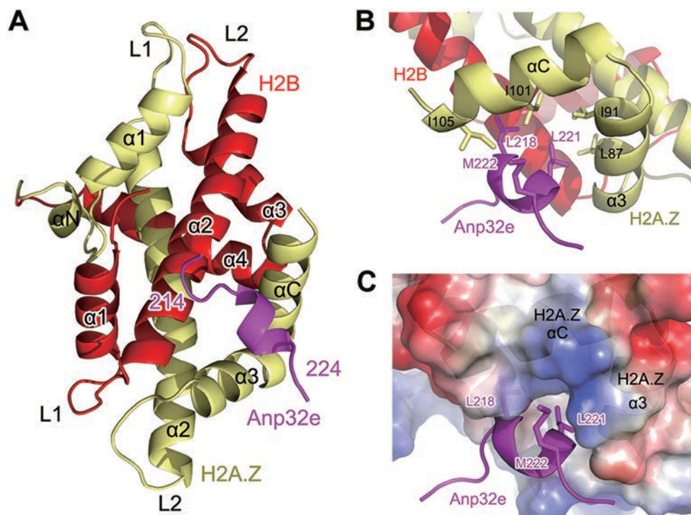
Figure 4 The structure of Anp32e in complex with H2B-H2A.Z. (A) The overall structure of the Anp32e 186-232 -lnkH2B-H2A.Z complex. The sequence of the observable part of Anp32e in the structure is 214 EEVGLSYLMKE 224 . (B) Major interactions between Anp32e 214-224 and H2A.Z α3 and αC helices. (C) Complementary surfaces between Anp32e 214-224 and H2A.Z α3 and αC helices
