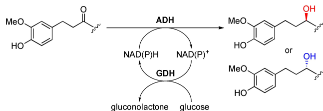
Scheme 1. General scheme of the biocatalyzed reduction of ginger active compounds ( 1 a–b , 3 and 4 ). The glucose/GDH system is used for cofactor regeneration.
