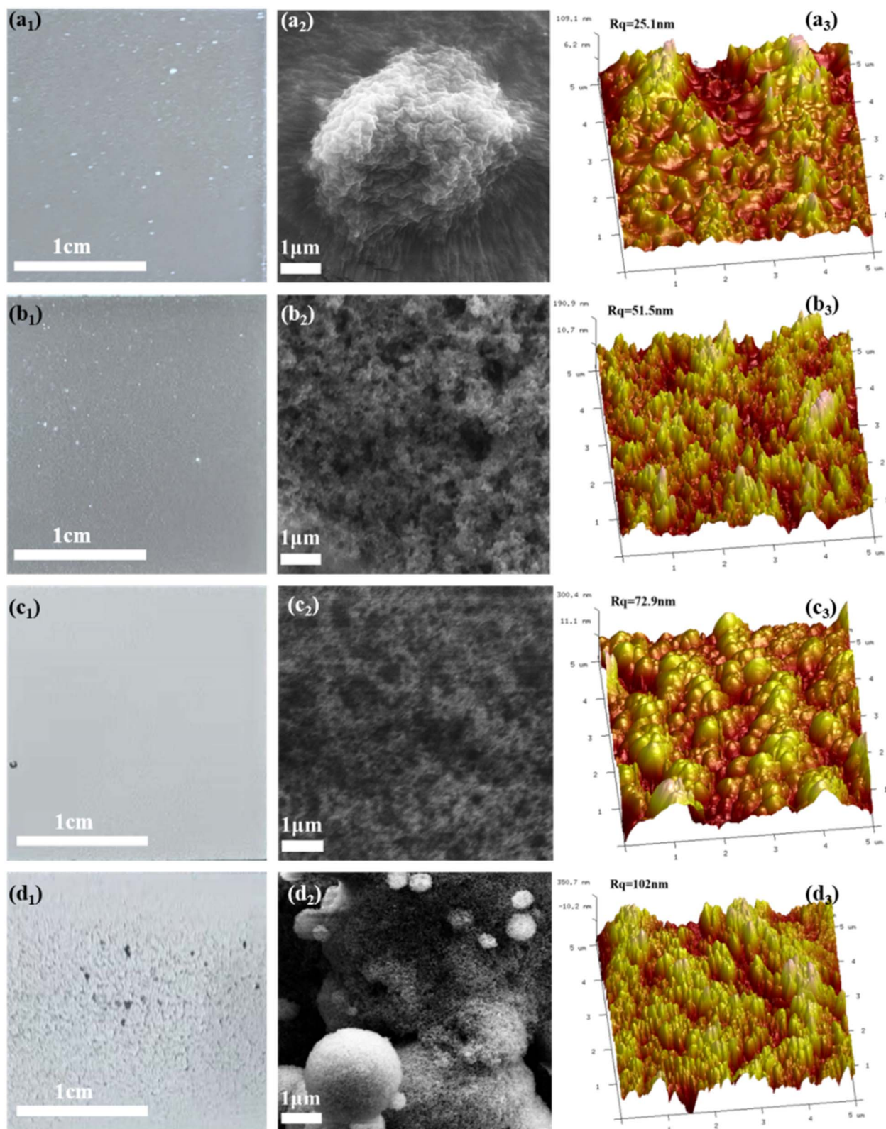
Fig. 4 The surface macro morphology, micro morphology and roughness of samples with different SiO 2 particle quality (a) 0.05 g (b) 0.1 g (c) 0.2 g (d) 0.4 g.
