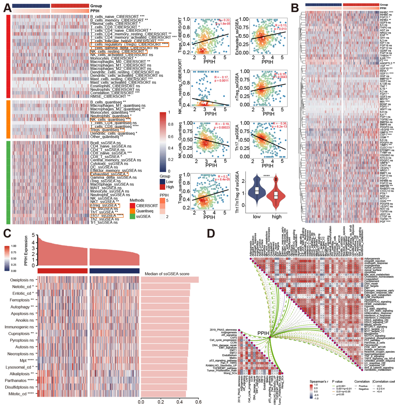
Figure 4 Associations of PPIH with the TME and cell death pathways in HCC. (A) Relationships between PPIH expression levels and infiltrating abundance were calculated via three algorithms: CIBERSORT, quantiseq and ssGSEA. A redder colour in the scatter plot indicates denser points. (B) Relationships between the PPIH expression levels and 83 EMT-associated growth factors. (C) Relationships between the PPIH expression levels and enrichment scores of 18 cell death-related gene sets. (D) Relationships between the PPIH expression levels and specific features, including published pathways and hallmark pathways. CCRI: cytokine–cytokine receptor interaction. “ns”: not significant; * P < 0.05 ; ** P < 0.01 ; *** P < 0.001 ; **** P < 0.0001 .
