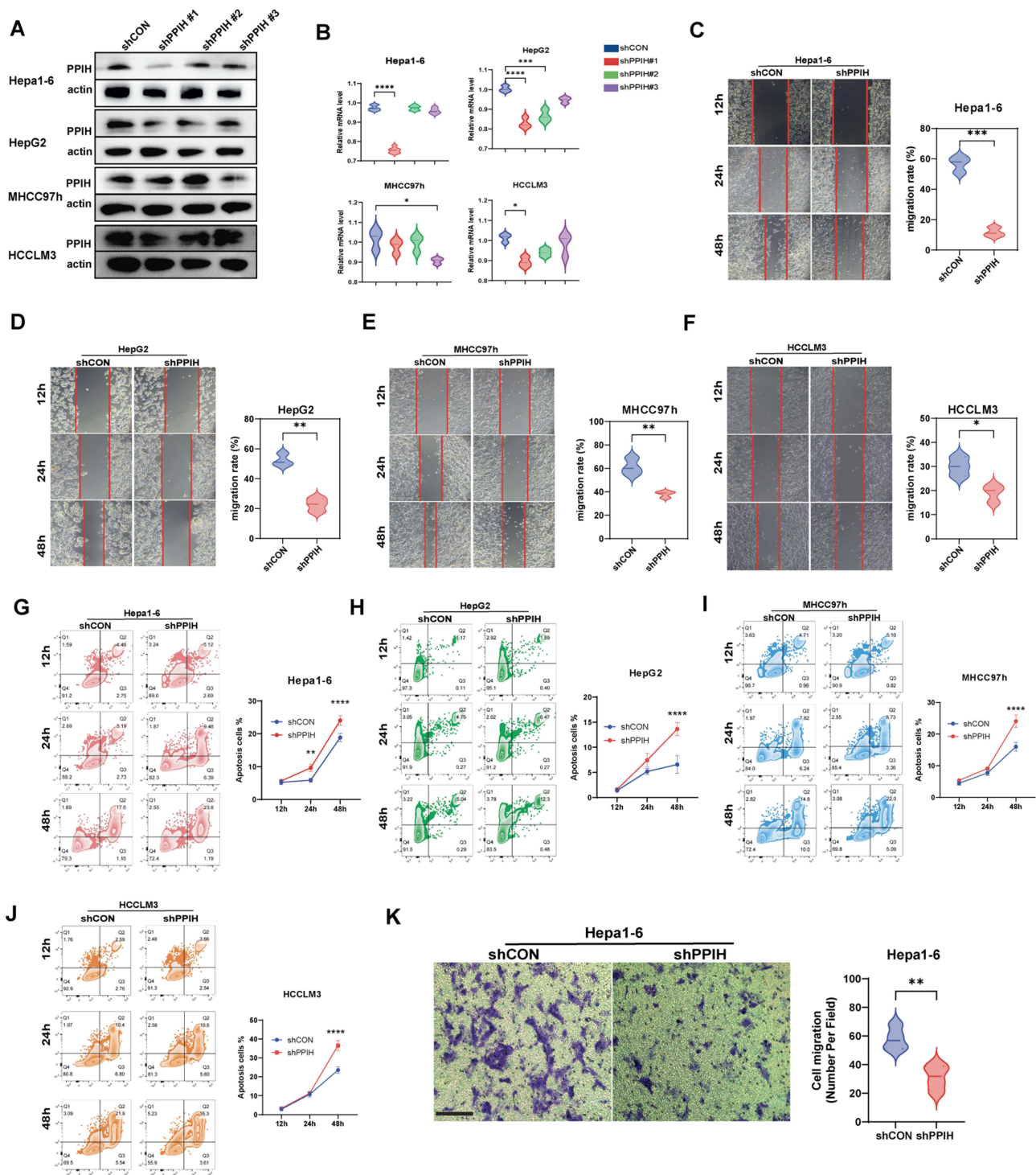
Figure 8 PPIH knockdown inhibits HCC cell proliferation, migration and invasion. (A) Western blotting confirmed the successful knockdown of PPIH by PPIH-specific shRNA in Hepa1-6, HepG2, MHCC97h and HCCLM3 cells. (B) Quantitative PCR analysis of the efficiency of PPIH knockdown in Hepa1-6, HepG2, MHCC97h and HCCLM3 cells. n = 3 . (C-F) Cell migration in the scratch assay. (G-J) PPIH knockdown induced apoptosis in different HCC cell lines, which increased with time. (K) Transwell invasion assay using a transwell chamber before and after PPIH knockdown. n = 4 , *P < 0.05 , **P < 0.01 , ***P < 0.001 , and ****P < 0.0001 indicate statistical significance compared with the control.
