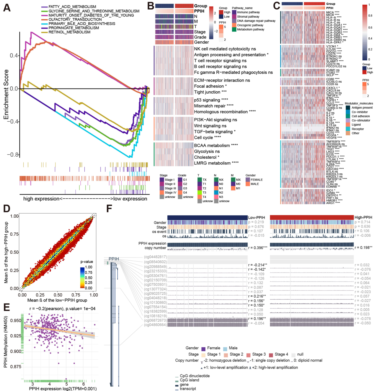
Figure 5 Differences in immune signatures and PPIH methylation between the low- and high-PPIH subgroups in HCC. (A) GSEA results demonstrate pathways notably enriched in both subgroups. (B) Enrichment levels of immune- and metabolism-associated pathways in both subgroups. (C) Heatmap of immunomodulatory factor expression in both subgroups. (D) Visualization of genes associated with differences in methylation. Each dot represents a gene. (E) Scatterplot of the correlation between PPIH methylation \beta values and PPIH expression. (F) Association between PPIH expression levels and methylation in both subgroups. "ns": not significant; * P < 0.05 ; ** P < 0.01 ; *** P < 0.001 ; **** P < 0.0001 .
