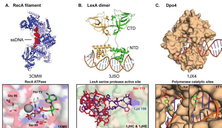
Figure 4. Targets of the SOS pathway. (A) Structure of the SOS sensor, RecA, shown as a filament (PDB entry 3CMW), with alternating monomers colored dark or light blue. The ssDNA is shown as red spheres. The panel below is a close-up of the ATP binding pocket (PDB entry 1XMS), a site that could be targeted. (B) Shown is dimeric LexA, bound to SOS box DNA (PDB entry 3JSO), with individual monomers colored green and yellow. The C-terminal protease domain (CTD) is connected to the N-terminal DNA binding domain (NTD) by a structurally unresolved linker (dashed line). In the self-cleavage mechanism, LexA undergoes a large conformational change in its C-terminal domain between inactive (red sticks, PDB entry 1JHC) and active states (purple sticks, PDB entry 1JHE) that positions the cleavage loop within the active site, adjacent to the Ser/Lys dyad. The overlaid active and inactive conformations are shown in the bottom panel. (C) Shown is a representative Y-family polymerase, Dpo4, an error-prone polymerase, bound to DNA (PDB entry 1JX4). Unlike high-fidelity T7 polymerase, shown for comparison (PDB entry 1T7P), Dpo4 possesses a more open, exposed catalytic site, which reduces the selectivity for the incoming nucleotide, colored green.
