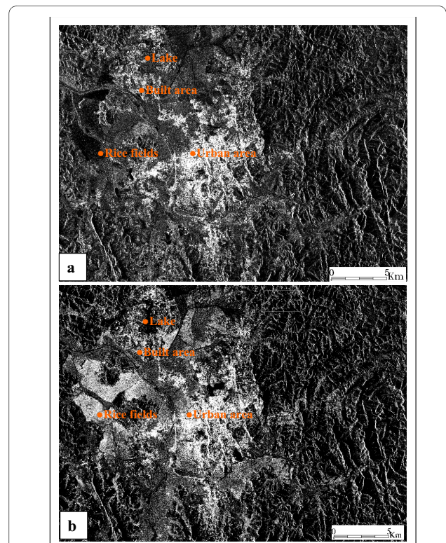
Figure 3 ASAR_IMP_1P images illustrating changes between January and July 2004. Difference between images acquired in January and July 2004.
