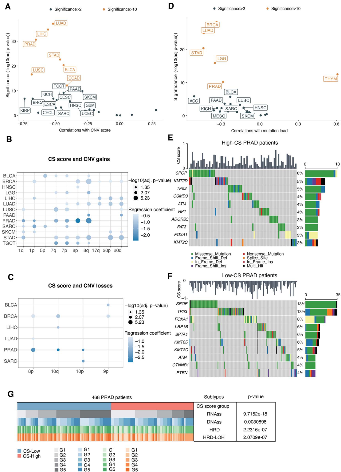
Figure 2. Associations between senescence levels and genomic variations at the pan-cancer level. (A) Associations between CS scores and CNV scores across TCGA cancer types (dots). Spearman correlations and significance [ -\log_{10}(\text{Benjamini-Hochberg-adjusted } P\text{-values}) ] are shown on the x-axis and y-axis. Labeled are significant CS-related cancers (significance > 2 ), and colored are those with significance > 10 . (B and C) Dot plots showing the associations between CS scores and arm-level CNV gains (B) and CNV losses (C) . Circle size indicates significance [ -\log_{10}(\text{Benjamini-Hochberg-adjusted } P\text{-values}) ], and the circle color denotes coefficients in multiple logistic regression. (D) Associations between CS scores and mutation loads across TCGA cancer types (dots). (E and F) Heatmap showing the top mutation events for individual TCGA PRAD patients in the high-CS (E) and low-CS groups (F) , respectively. Bar plots in the top panel represent the CS scores of individual patients. Statistical graph of mutation events for each gene is shown in the left panel. Colors are variant classifications. (G) Comparative analysis of different PRAD subtypes. Cochran-Mantel-Haenszel test P-values are stated. PRAD patients were classified into five equal subtypes (G1–G5, from the 20% to 80% quantile) based on the range of RNAss, DNAss, HRD and HRD-LOH, respectively.
