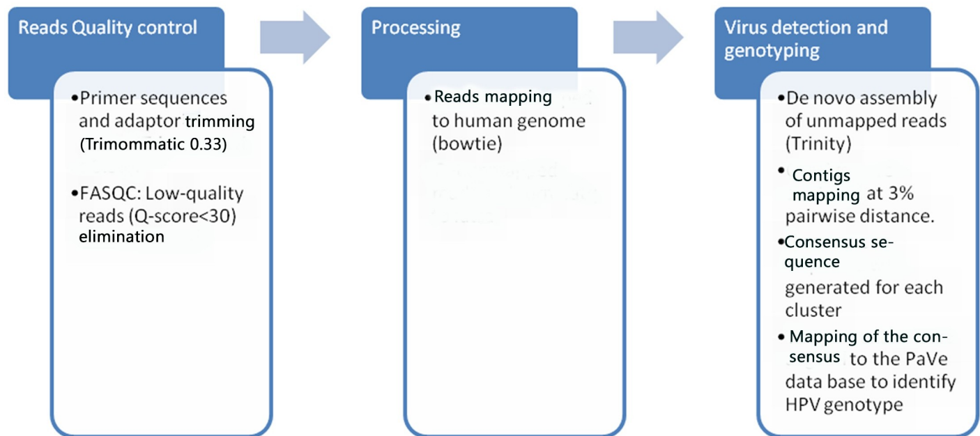
Fig 2. Workflow for data analysis. The designed pipeline for HPV genotyping in this study contains 3 steps: reads quality control to remove bad quality reads, processing of retained reads for mapping into Human genome, and finally in the final set of selected sequences the viruses were detected and genotyped by assembly and contigs mapping to HPV reference genome.
