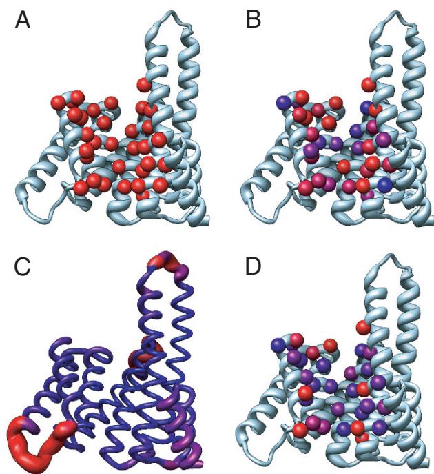
Figure 7 Peptide binding residues of 14-3-3 \zeta . (A) The C \beta atoms of all residues involved in binding in any of the five peptide bound structures are shown (red) along with the rest of the backbone (light blue ribbon). (B) The standard deviation in the area bound on complex formation is displayed by coloring the C \beta atoms of peptide binding residues on a gradient, from a standard deviation of 0Å 2 (blue) to 10Å 2 and greater (red). (C) The backbone RMSF of the 14-3-3 domain calculated over C \alpha atoms displayed as a color and radius gradient, from an RMSF of 0Å (blue, 0.25Å) to an RMSF of 2.0Å and greater (red, 2.0Å). (D) The side chain RMSF is displayed by coloring the C \beta atoms of peptide binding residues on a gradient, from a RMSF of 0Å (blue) to an RMSF of 0.50Å and greater (red). All parameters were calculated using all five of the peptide-14-3-3 complexes.
