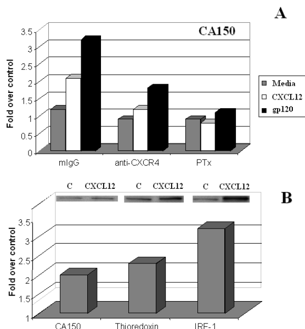
Figure 7 CA150/TCERG1, thioredoxin and IRF-1 protein expression by Jurkat T cells post CXCL12 \alpha treatment. Jurkat cells were treated for 24 hrs with either CXCL12 (A, B) or gp120 IIIB (A) at 1 \mu g/ml in the presence or absence of control mouse IgG, mouse anti-human CXCR4 mAb, or pertussis toxin (PTx; 200 ng/ml) at 37°C. After incubation, the cell pellets were isolated, counted, washed, and subsequently lysed with the detergent. Protein determinations were then performed. Samples were loaded at 20 \mu g per lane on a 10% polyacrylamide gel. After electrophoresis, the gels were transferred using a transfer apparatus to an immobilon membrane and stained for CA150/TCERG1 (A, B), thioredoxin (B) or IRF-1 (B) expression via Western blot analysis (shown in panel B for each of these proteins versus control). The results are expressed as fold change versus control expression (post background subtraction).
