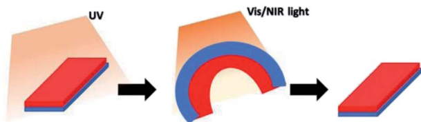
Fig. 5 The schematic illustration of shape memory of the bilayer film consisting of AZO-PU and EVA composites upon UV/Vis/NIR light irradiation (red: AZO-based PU layer and blue: EVA composite with photothermal filler layer).
