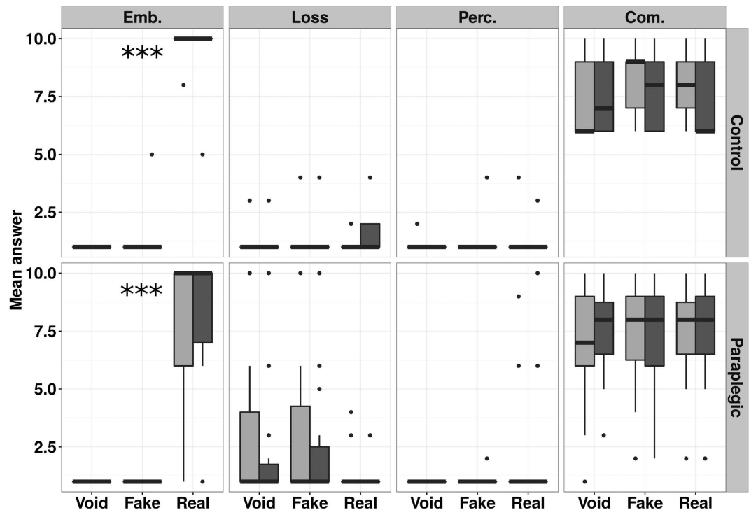
Figure 3. Experiment 1 - CCE around the feet, Boxplot of questionnaire data. The graph is organised in a matrix: the Components (Emb. = Embodiment of own feet, Loss = Loss of own feet, Perc. = Perceived Movements and Com. = Compliance) are in the columns and the groups (Control group and Paraplegic group) are in the horizontal rows (top and bottom). The timing (Before – lighter grey and After – darker grey) and the experimental conditions (Fake, Real, Void) are represented side by side for ease of comparison. The values are as in Fig. 2. The boxes with “***” represent the conditions where there were different subjective “Embodiment of own feet” sensations among conditions.
