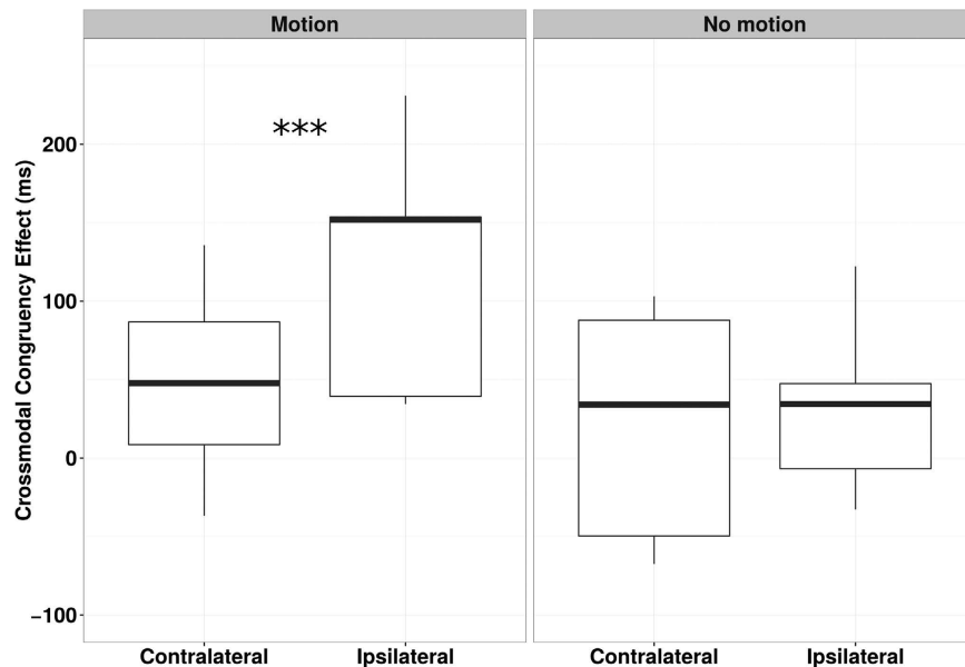
Figure 5. Experiment 3 - CCE around the feet after passive motion, Box plot of CCE data. The graph is organised in columns with the Motion group on the left and the No-motion group on the right. Contralateral and Ipsilateral data are side by side in order to facilitate interpretation. Means and standard deviations for the CCE: Motion Contralateral = 48.19 \pm 60.30 ; Motion Ipsilateral = 114.78 \pm 77.19 ; No-motion Contralateral = 20.87 \pm 75.46 ; No-motion Ipsilateral = 0.43 \pm 96.76 . The box with “***” represents the condition where Contralateral and Ipsilateral CCEs were different according to the SPM and frequentist (see SM, S4.1) statistics.
