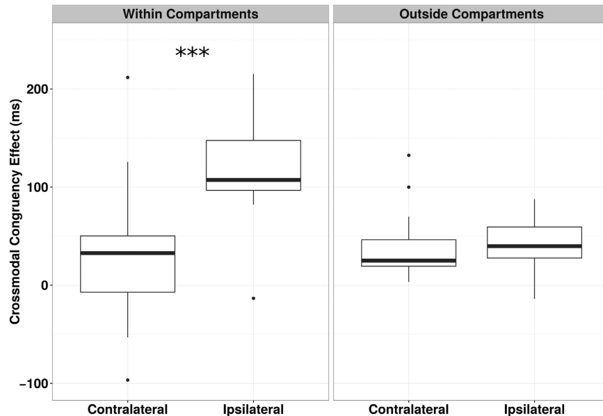
Figure 4. Experiment 2 - CCE around the hands, Box plot of CCE data. The graph is organized as a matrix: the Conditions (Within Compartments, Outside Compartments) are in the columns, Contralateral and Ipsilateral data are side by side in order to facilitate interpretation. Means and standard deviations for the CCE: Within Compartments Contralateral = 36.94 \pm 77.89 ; Within Compartments Ipsilateral = 122.88 \pm 58.99 ; Outside Compartments Contralateral = 57.21 \pm 132.16 ; Outside Compartments Ipsilateral = 40.51 \pm 88.96 . The box with “***” represents the condition where Contralateral and Ipsilateral CCEs were different according to the SPM and frequentist (see SM, S4.1) statistics.
