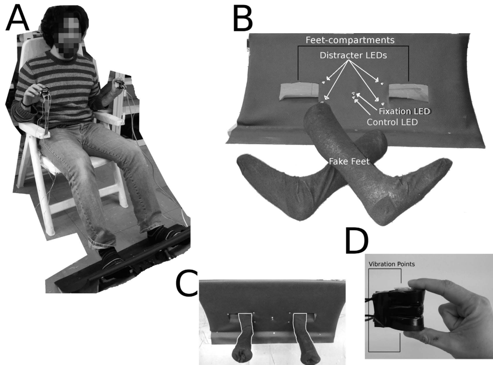
Figure 1. (A) Experimental set up. Typical position of a participant for the Real condition in Experiment 1 and Experiment 3. Note the participant's feet within the feet-compartments of the wooden frame. (B) Wooden frame with fake feet and LEDs position. (C) Wooden frame with fake feet inserted into the feet compartments. (D) Tactile stimulators where vibration is delivered against the index (high position) or the thumb finger (low position).
