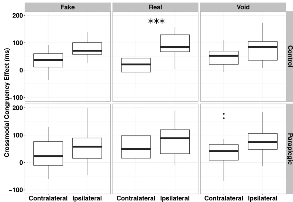
Figure 2. Experiment 1 - CCE around the feet, Boxplot of CCE data. The graph is organised as a matrix: the Conditions (Fake, Real, Void) are in the columns and the groups (Control group and Paraplegic group) are in the horizontal rows (top and bottom). Contralateral and Ipsilateral data are side by side in order to allow direct comparisons. The darker line in the middle of the box is the median, the box represents the first and the third quartile and the bottom and top whiskers represents respectively the first quarter minus 1.5 \times Interquartile Range and the third quarter plus 1.5 \times Interquartile Range. The means and standard deviations for the CCE of the Control group are: Fake Contralateral = 35.43 \pm 32.78 ; Fake Ipsilateral = 77.52 \pm 31.65 ; Real Contralateral = 20.56 \pm 41.53 ; Real Ipsilateral = 92.86 \pm 43.49 ; Void Contralateral = 47.62 \pm 33.83 ; Void Ipsilateral = 77.86 \pm 41.66 . The means and standard deviations for the CCE of the Paraplegic group are: Fake Contralateral = 29.38 \pm 53.21 ; Fake Ipsilateral = 81.93 \pm 88.91 ; Real Contralateral = 52.43 \pm 57.79 ; Real Ipsilateral = 88.96 \pm 63.71 ; Void Contralateral = 46.73 \pm 57.67 ; Void Ipsilateral = 90.88 \pm 62.89 . The box with “***” represents the condition where Contralateral and Ipsilateral CCEs were different according to the SPM and frequentist (see SM, S4.1) statistics.
