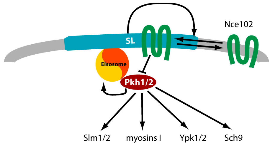
Figure 10. Model for Nce102 function in sphingolipid sensing. Nce102 (green) senses sphingolipid levels in the plasma membrane by distributing between the thick sphingolipid-rich MCC (blue) and the rest of the plasma membrane (gray) depending on sphingolipid levels. In the MCC, it inhibits Pkh kinases (red) that localize under this domain at eisosomes.
