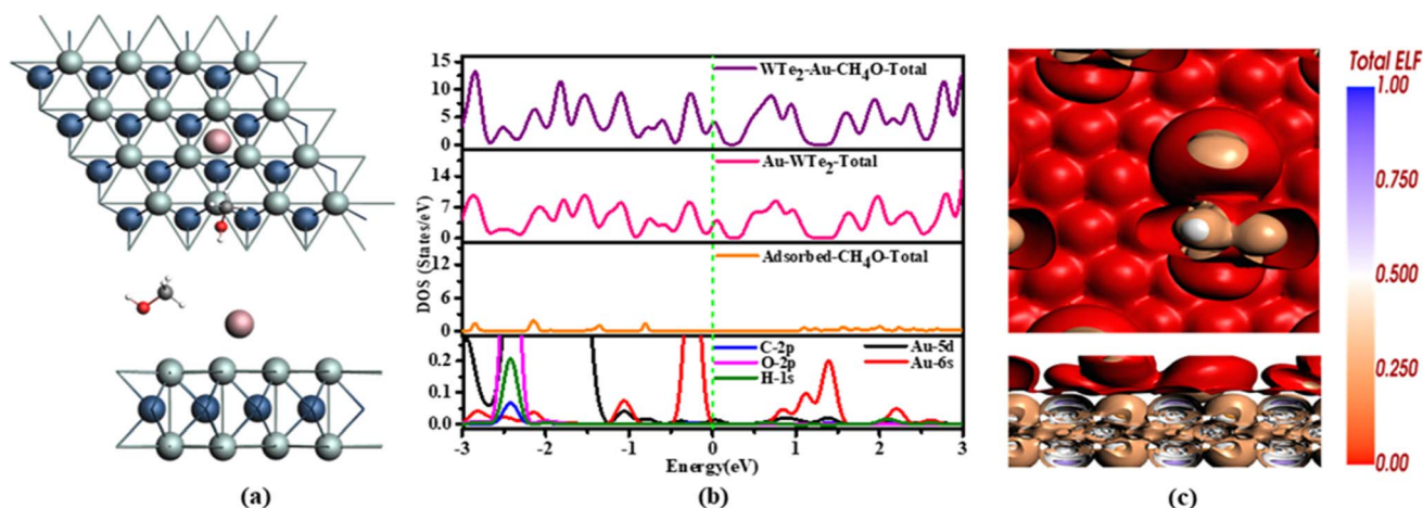
Fig. 8 (a) Configuration of \text{CH}_4\text{O} adsorption (b) TDOS and PDOS (c) ELF of \text{CH}_4\text{O} .
