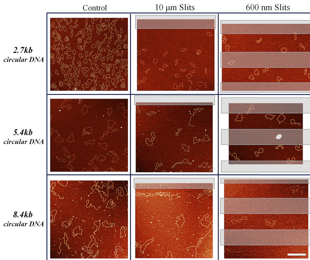
Figure 3. Large scale AFM images of three types of circular DNA (2.7, 5.4 and 8.4 kb) versus slit size. Left column shows control measurements; middle column shows DNA inside 10 \mu\text{m} giant slits; right column shows DNA inside 600 nm small slits. Transparent rectangles represent places where the slits were placed. DNA molecules outside the slits were not included in the statistics. Scale bar: 1 \mu\text{m} .
