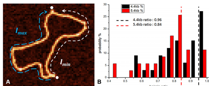
Figure 6. (A) Defining DNA hairpin ratio by measuring the ratio between the minimal and the maximal arc length along the DNA between two hairpins. (B) The hairpin arc ratio distribution for 4.4 kb (black bars) and 5.4 kb (red bars) nicked DNA. Red and black dotted lines represent the positions of the nicked sites.
