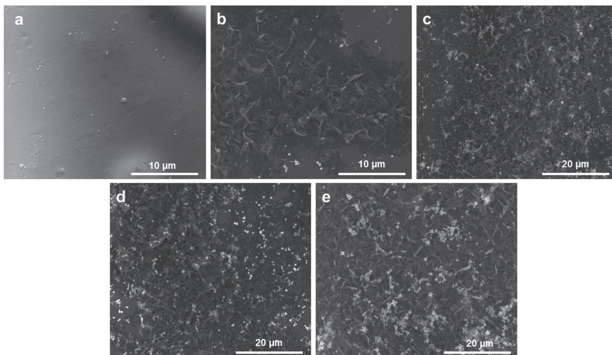
Figure 4 SEM images of Gly-His film structures kept in \text{AgNO}_3 solution for a) 0 h, b) 3 h, c) 6 h, d) 12 h, and e) 24 h
