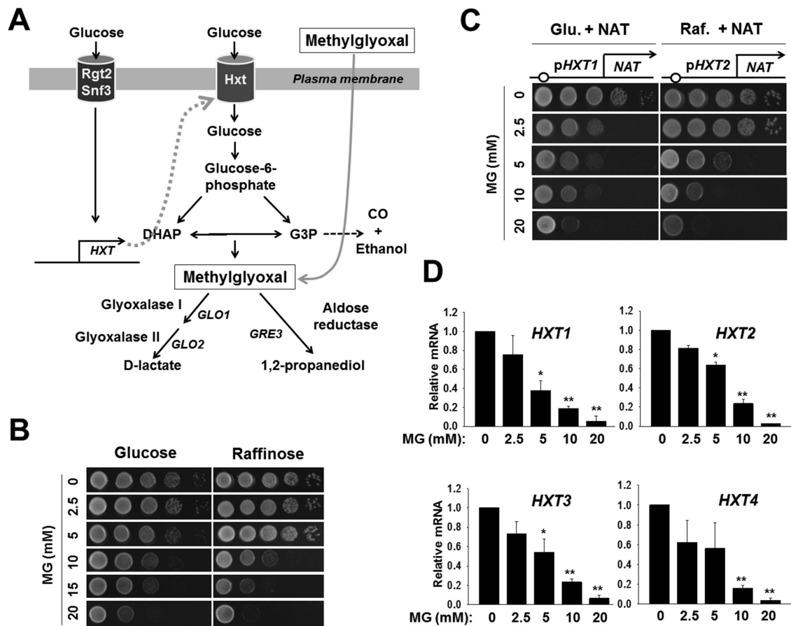
FIGURE 1: Methylglyoxal inhibits expression of the HXT genes. (A) Schematic representation of MG metabolism pathways. MG is produced as a by-product of glycolysis by degradation of the triose phosphates DHAP and G3P. It is then metabolized into D-lactate by glyoxalase systems ( GLO1 and GLO2 ) or 1,2-propanediol by aldolase reductase ( GRE3 ). (B) Yeast cells ( WT ) were spotted on YP plates containing 2% glucose (Glucose) or 2% raffinose (Raffinose) supplemented with different concentrations of MG as shown. The first spot of each row represents a count of 5 \times 10^7 cells/ml, which is diluted 1:10 for each spot thereafter. The plates were incubated for 2 d and photographed. (C) HXT-NAT reporter strains were spotted on YP plates containing 2% glucose (Glu. + NAT) or 2% raffinose (Raff. + NAT) supplemented with 100 \mu g/ml NAT sulfate and the indicated concentrations of MG, as described in B. The plates were incubated for 2 d and photographed. (D) qRT-PCR analysis of mRNA expressions of HXT1 , HXT2 , HXT3 , and HXT4 genes. mRNA was isolated from yeast cells ( WT ) grown in either 2% glucose (to quantify HXT1 and HXT3 gene expressions) or 2% raffinose (to quantify HXT2 and HXT4 gene expressions) containing the indicated amounts of MG. The data are averages of three independent experiments, with error bars showing mean \pm SD. * p < 0.05 and ** p < 0.001 .
