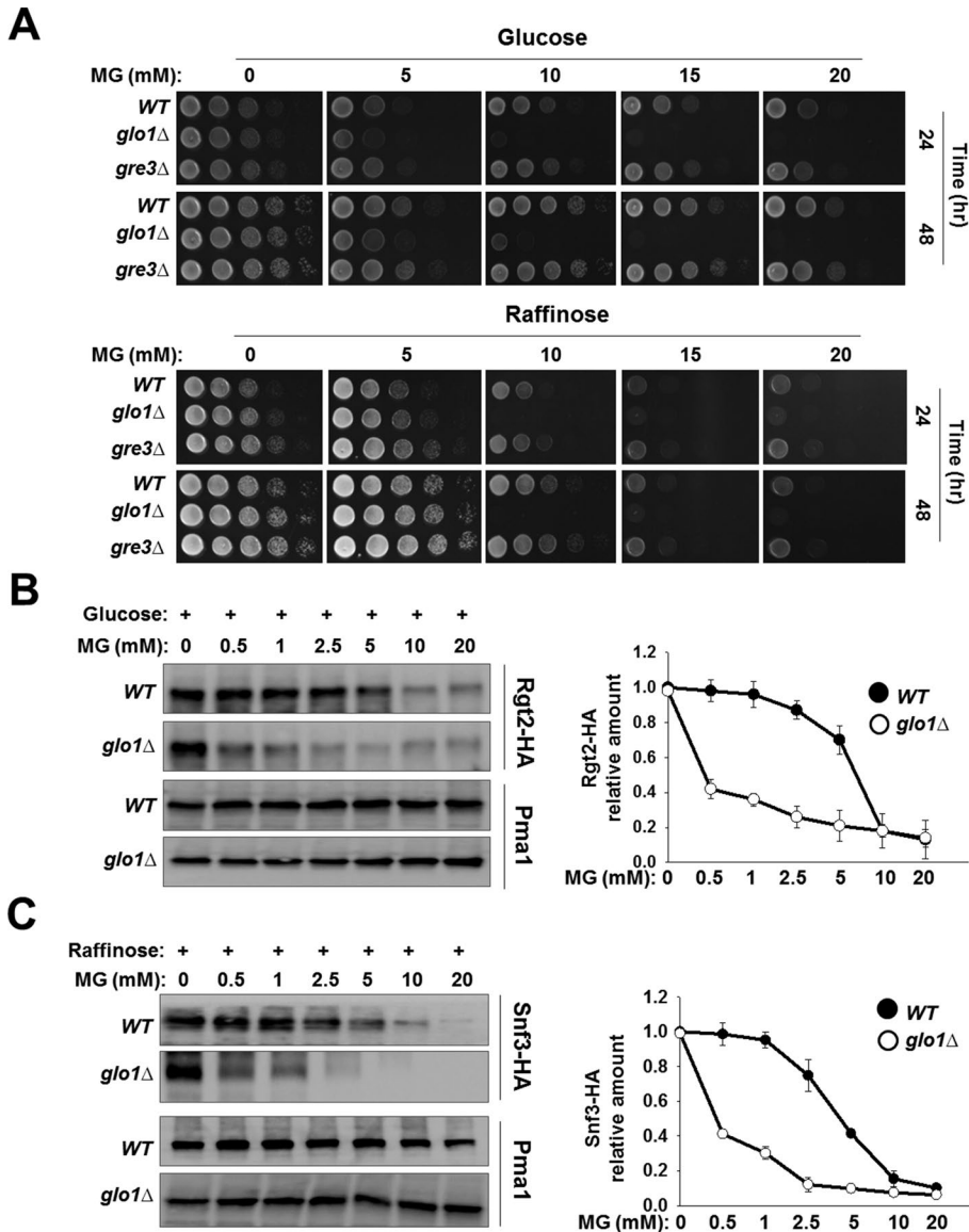
FIGURE 6: Inactivation of GLO1 gene causes rapid down-regulation of Rgt2 and Snf3. (A) Yeast cells (WT, glo1 Δ and gre3 Δ) were spotted on YP plates containing 2% glucose (Glucose) or 2% raffinose (Raffinose) supplemented with the indicated concentrations of MG, as described in Figure 1B. The plates were incubated for the indicated time and photographed. (B) Western blot analysis of Rgt2-HA at the plasma membrane. Yeast cells (WT and glo1 Δ) expressing Rgt2-HA were grown in SC medium containing 2% glucose until mid log phase and treated with the indicated concentrations of MG for 2 h. Membrane fractions were immunoblotted with anti-HA and anti-Pma1 antibodies (left). (C) Western blot analysis of Snf3-HA at the plasma membrane. Yeast cells (WT and glo1 Δ) expressing Snf3-HA were grown in SC medium containing 2% raffinose until mid log phase and treated with the indicated concentrations of MG for 2 h. Membrane fractions were immunoblotted with anti-HA and anti-Pma1 antibodies (left). The intensities of each band on the blots in B and C were quantified by densitometric scanning (right). Pma1 served as a loading control in B and C.
