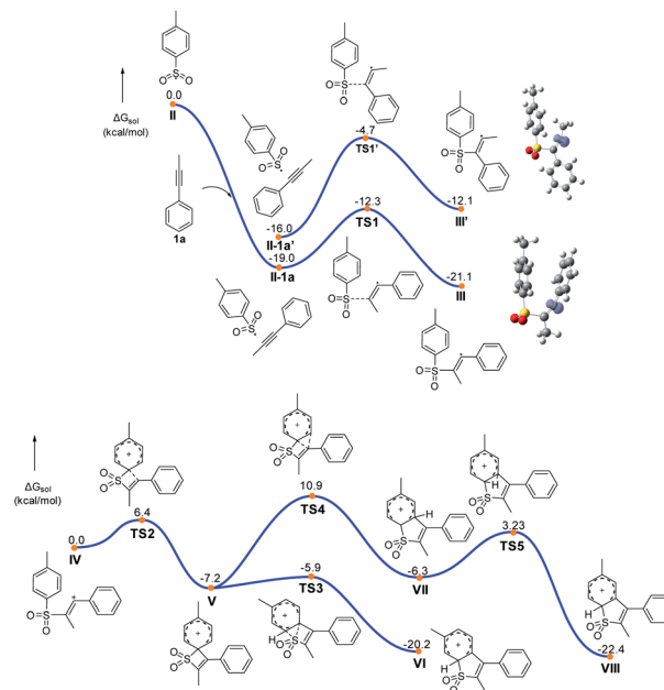
Fig. 2 DFT calculations.
