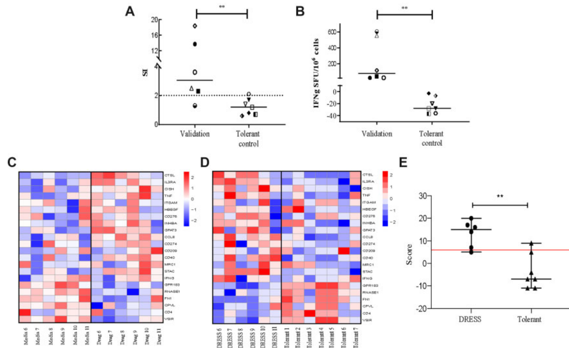
Figure 5. DRESS validation cohort confirms specificity of biomarker panel. A–B, Characteristics of in vitro responses to culprit drug in antibiotic-DRESS validation cohort ( n=6 ) and control patients tolerant of similar antibiotics ( n=7 ). A, Lymphocyte proliferation test (LPA) measured as stimulation index (SI) of proliferation induced by drug versus media control. B, IFN- \gamma release in drug-induced responses measured by ELISpot. Each data point represents maximum measured response to tested drug. Horizontal solid lines indicate group median. Horizontal dotted line shows positive result threshold. Mann-Whitney U test used for statistical significance (** = p < .01 ). C, Heatmap depicting changes in expression of selected 22 candidate biomarkers in validation DRESS cohort exposed to culprit drug versus media control. Color indicates the expression change in logFC. Red: upregulated genes; blue: downregulated genes. D, Heatmap depicting changes in expression of selected 22 candidate biomarkers in validation DRESS cohort versus tolerant patients. Color indicates the expression change in logFC. Red: upregulated genes, blue: downregulated genes. E, Box and whisker plot showing cumulative scoring using 22 biomarker genes compared with expected expression alterations based on signature panel. Error bars indicate data range. Horizontal red line indicates threshold score considered positive. (** = p < .01 , Fisher's exact test). Abbreviations: IFN- \gamma ELISpot, interferon-gamma enzyme-linked immunosorbent spot; SFU, spot forming unit. A color version of this figure appears in the online version of this article.
