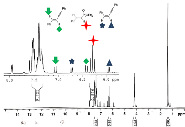
Fig. 1 ^1\text{H} NMR spectrum of the reaction mixture of 1a in \text{CDCl}_3 .
