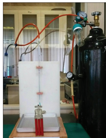
Figure 1: Fluid infiltration system.
