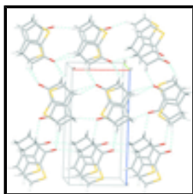
Fig. 3. A general view of the crystal packing for the title compound with hydrogen bonds drawn as dashed lines.
