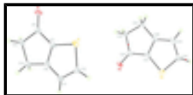
Fig. 1. The asymmetric unit of I with ellipsoids drawn at the 50% probability level.
