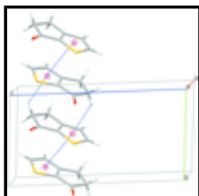
Fig. 2. \pi - \pi and C-H... \pi contacts forming columns along b , with contacts shown as dashed lines.
