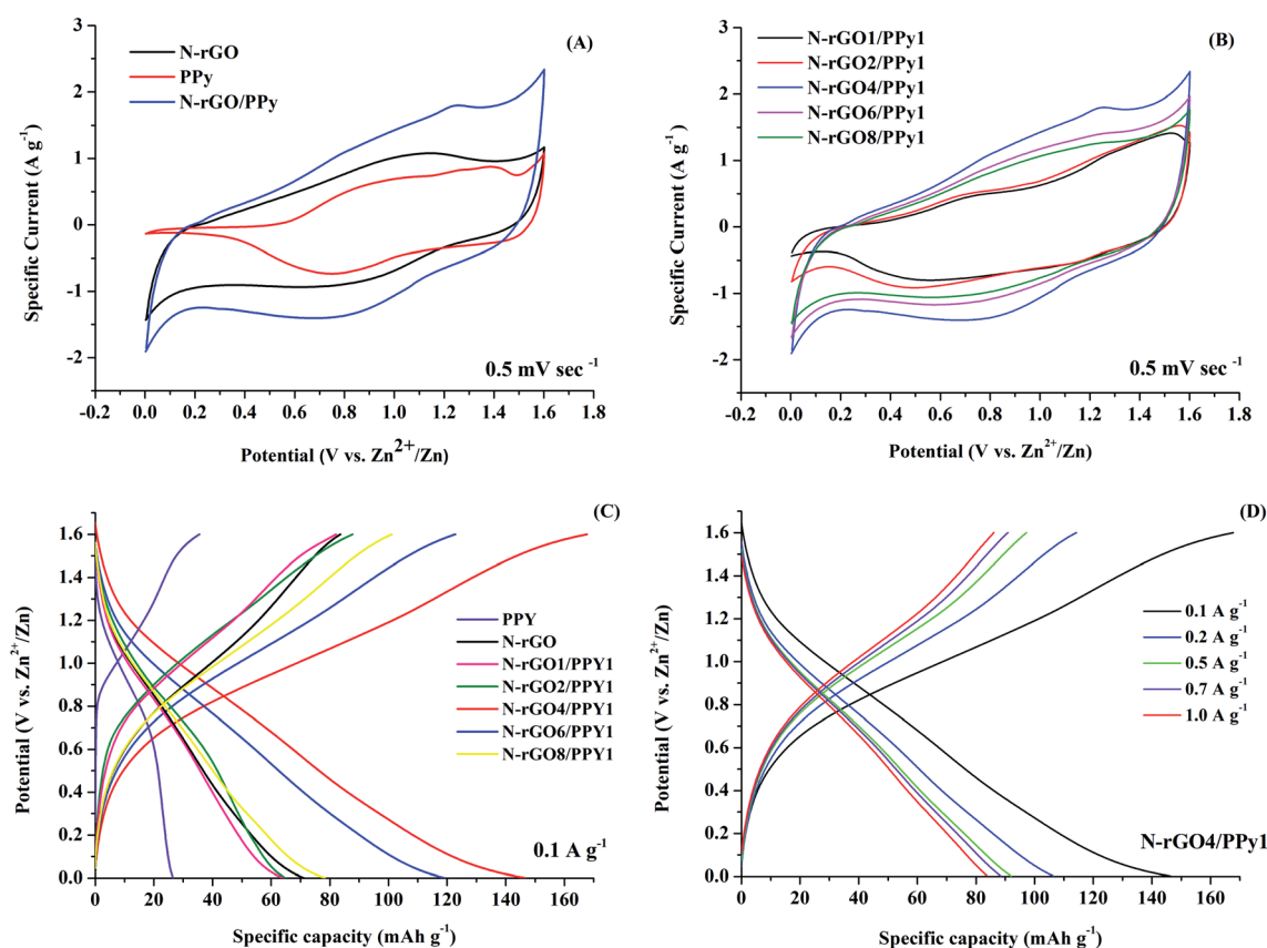
Fig. 7 Cyclic voltammograms results in 0.2 M \text{ZnSO}_4 for (A) PPy, N-rGO, and N-rGO1/PPy1 at 0.5 \text{ mV s}^{-1} , and (B) N-rGO/PPy1 samples with various N-rGO/PPy ratios at 0.5 \text{ mV s}^{-1} ; galvanostatic charge–discharge profiles for 3rd cycle of (C) N-rGO/PPy1 samples with various N-rGO/PPy ratios at 0.1 \text{ A g}^{-1} , and (D) N-rGO4/PPy1 at various current density.
