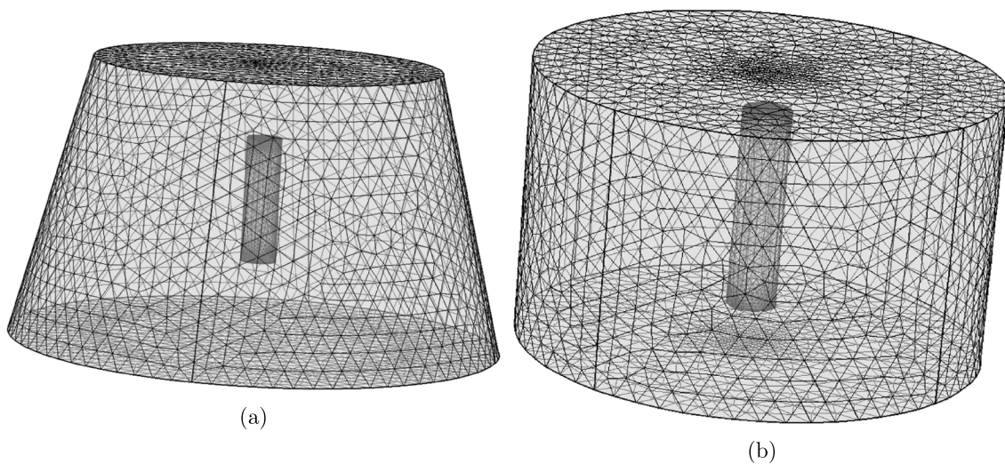
Fig. 4 (a) FEM mesh generated for the 3D 8-orifice pin geometry for the influence of flow study. Mesh consists of 217,071 domain elements, 10,434 boundary elements, and 928 edge elements. A similar mesh for the 2-orifice pin was also created which consisted of 178,296 domain elements, 9050 boundary elements, and 728 edge elements. (b) FEM mesh generated for the 3D porous pin geometry for the influence of flow study. Mesh consists of 243,870 domain elements, 8652 boundary elements, and 652 edge elements.
