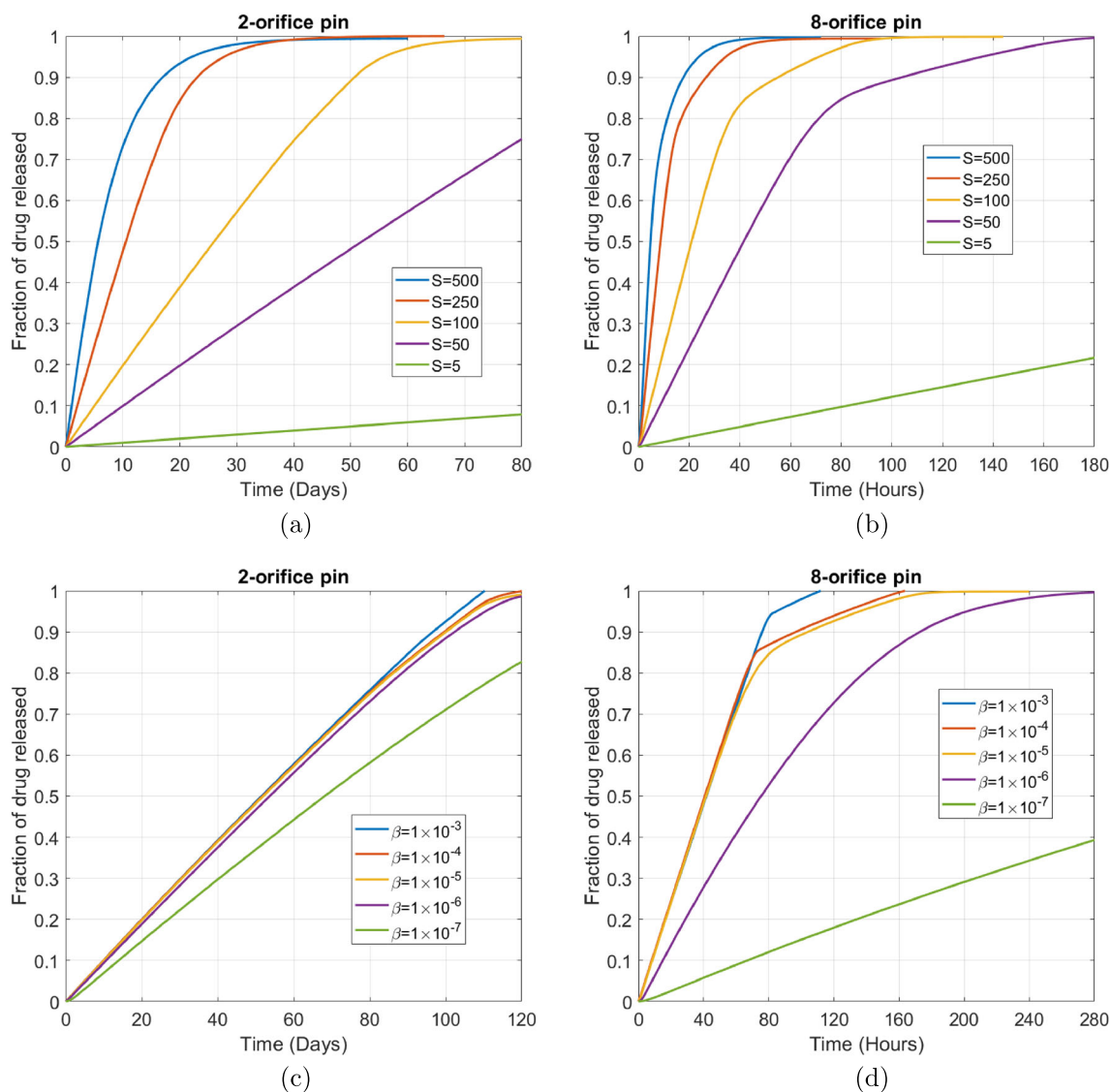
Fig. 12 Plots showing the effect of varying the drug solubility S for (a) the 2-orifice pin and (b) the 8-orifice pin. Plots showing the effect of varying the dissolution rate \beta for (c) the 2-orifice pin and (d) the 8-orifice pin. The remaining parameters are the baseline parameters as stated in Table 2. The fraction of drug released was calculated using M_{rel}(t) = \int_{\Omega_1} c d\Omega_1 / b_0 \int_{\Omega_3} d\Omega_3 .
