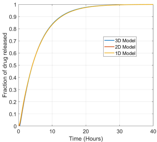
Fig. 9 Plot showing fraction of drug released for the porous pin for the 1D, 2D and 3D diffusion models using the relevant baseline parameters from Table 2. The fraction of drug released in the case of the 3D model was calculated using M_{rel}(t) = 1 - (\int_{\Omega_3} c_d d\Omega_3 + \int_{\Omega_2} c_p d\Omega_2) / b_0 \int_{\Omega_3} d\Omega_3 .
