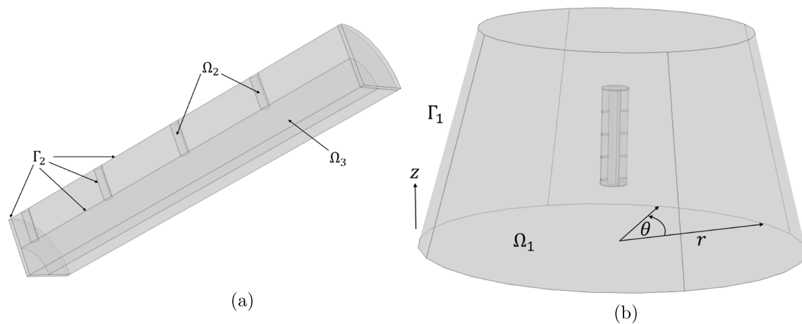
Fig. 2 (a) A close-up of a segment of the 8-orifice pin, clearly showing the drug core \Omega_3 and the collection of orifices \Omega_2 , which extend through the wall of the pin. \Gamma_2 represents the entire surface area of the pin, including the cylindrical walls of the orifices in each pin configuration. (b) Geometrical configuration of the 8-hole pin within a section of a conical flask. The release medium fluid is represented by \Omega_1 . The set of boundaries between the release medium and the flask are collectively represented by \Gamma_1 . The default Cartesian (x,y,z) co-ordinate system within COMSOL Multiphysics®, version 5.3a, was employed, with the origin located at the centre of the flask base and the z -axis pointing vertically upwards. On the boundary \Gamma_1 , a moving wall boundary condition (2) is imposed to simulate stirring. For ease of implementation, a cylindrical co-ordinate system was employed for this boundary condition: r denotes the radius from the central z -axis to the outer wall and \theta is the angle which \Omega_1 makes with respect to its original position as it rotates.
