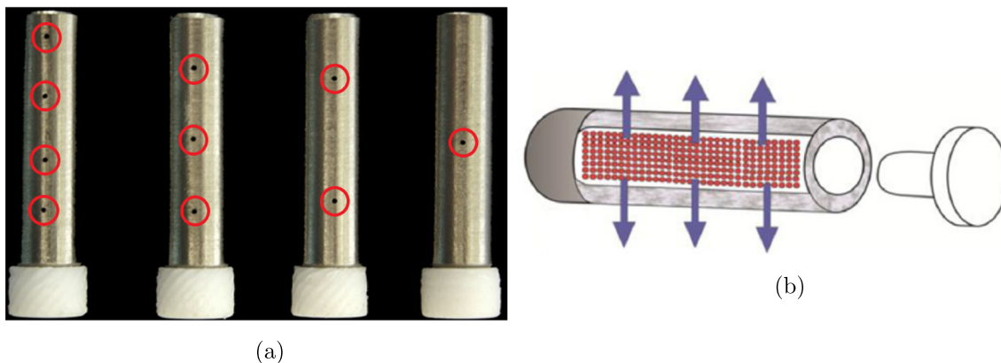
Fig. 1 (a) The orifice pins showing (left to right) 8, 6, 4 and 2 drilled holes, highlighted by the red circles, through which the drug is released (6). (b) Illustration of the porous pin with blue arrows showing drug transport through the porous wall (5).
