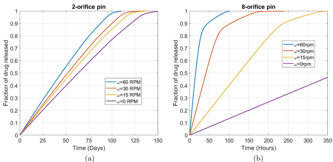
Fig. 10 Plots showing the effect of varying the rotational flow speed for (a) the 2-orifice pin and (b) the 8-orifice pin. The remaining parameters are the baseline parameters as stated in Table 2. The fraction of drug released was calculated using M_{rel}(t) = \int_{\Omega_1} c d\Omega_1 / b_0 \int_{\Omega_3} d\Omega_3 .
