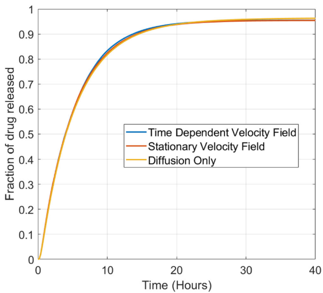
Fig. 7 Plot showing the effect of including fluid flow compared to a purely diffusive problem for the porous pin. The baseline free diffusive coefficient of D_f = 10^{-9} \text{ m}^2/\text{s} and rotation speed of \omega = 30 \text{ RPM} have been used to generate these plots. The fraction of drug released was calculated using M_{rel}(t) = \int_{\Omega} c_m d\Omega_1 / b_0 \int_{\Omega_3} d\Omega_3 .
