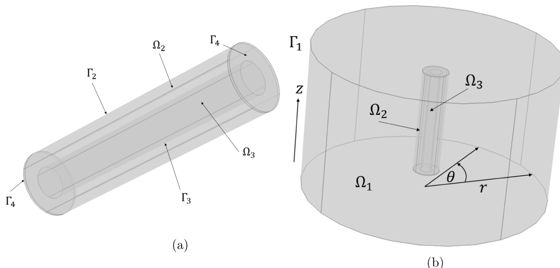
Fig. 3 (a) The 3D porous pin highlighting \Omega_2 (the porous wall) and \Omega_3 (the inner drug core). The outer boundary of the porous wall of the pin in contact with the release medium is denoted \Gamma_2 and the interface between the inner drug core and the porous wall is represented by \Gamma_3 . The collection of boundaries that form the top and bottom caps of the pin are designated by \Gamma_4 . (b) 3D geometry of the porous pin experimental set-up, where the domains \Omega_1 , \Omega_2 and \Omega_3 represent the release medium, the porous wall of the pin and the inner drug core of the pin, respectively. \Gamma_1 is the outer boundary of the release medium, \theta is the angle that \Omega_1 makes with respect to its original position as it rotates and r is the radius from the central z -axis to the outer wall.
