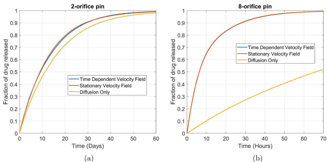
Fig. 5 (a) Plot showing the effect of including fluid flow compared to a purely diffusive problem for (a) the 2-orifice pin and (b) the 8-orifice pin. The baseline free diffusion coefficient of D_f = 10^{-9} \text{ m}^2/\text{s} and rotation speed of \omega = 30 \text{ RPM} have been used to generate these plots. The fraction of drug released was calculated using M_{rel}(t) = \int_{\Omega_1} c d\Omega_1 / b_0 \int_{\Omega_2} d\Omega_2 .
