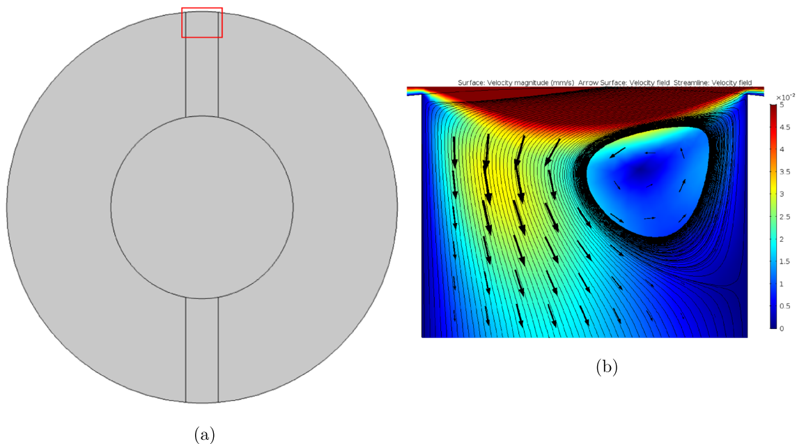
Fig. 6 (a) A horizontal cross-sectional slice through the centre of the top pair of orifices of the 8-orifice pin. (b) Image of the velocity field within the red box region of the cross-sectional slice. The baseline rotation speed of \omega = 30 \text{ RPM} has been used to generate this plot.
