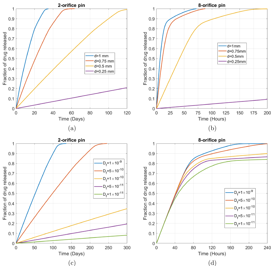
Fig. 11 Plots showing the effect of varying the orifice diameter d for (a) the 2-orifice pin and (b) the 8-orifice pin. Plots showing the effect of varying the drug free diffusion coefficient D_f for (c) the 2-orifice pin and (d) the 8-orifice pin. The remaining parameters are baseline parameters as stated in Table 2. The fraction of drug released was calculated using M_{rel}(t) = \int_{\Omega_1} c d\Omega_1 / b_0 \int_{\Omega_3} d\Omega_3
