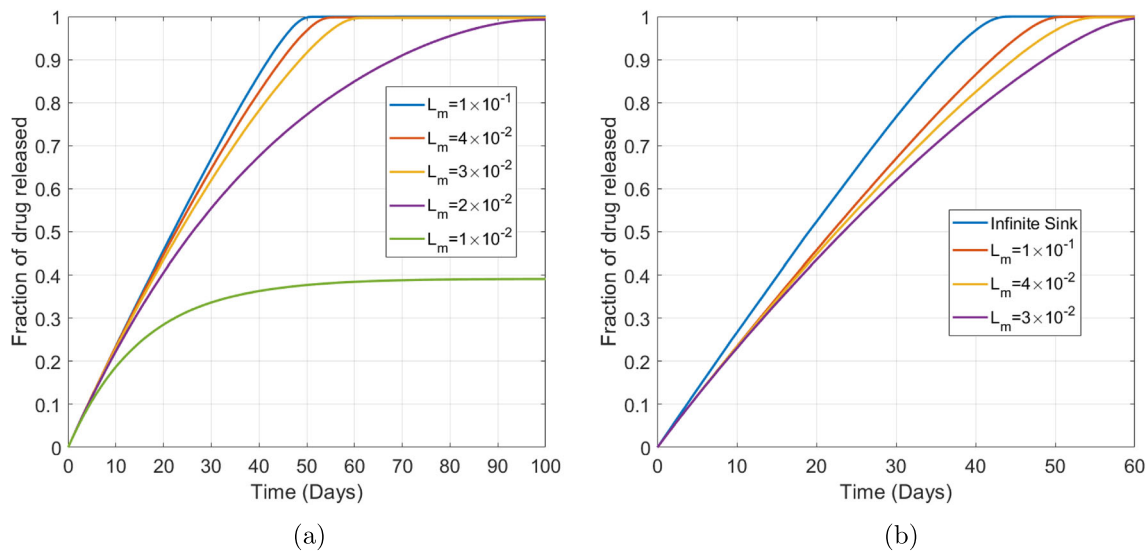
Fig. 14 Plots showing the effect of (a) varying the length scale of the release medium (b) approximating the release medium through an infinite sink boundary condition. The remaining parameters are baseline parameters as stated in Table 2. The fraction of drug released in all cases was calculated using M_{rel}(t) = \int_{(L_d+L_p)}^{(L_d+L_p+L_m)} c_m r dr / b_0 \int_0^{L_d} r dr , except for the infinite sink case where M_{rel}(t) = 1 - \left( \int_0^{L_d} c_d r dr + \phi \int_{L_d}^{(L_d+L_p)} c_p r dr \right) / b_0 \phi \int_0^{L_d} r dr was used.
