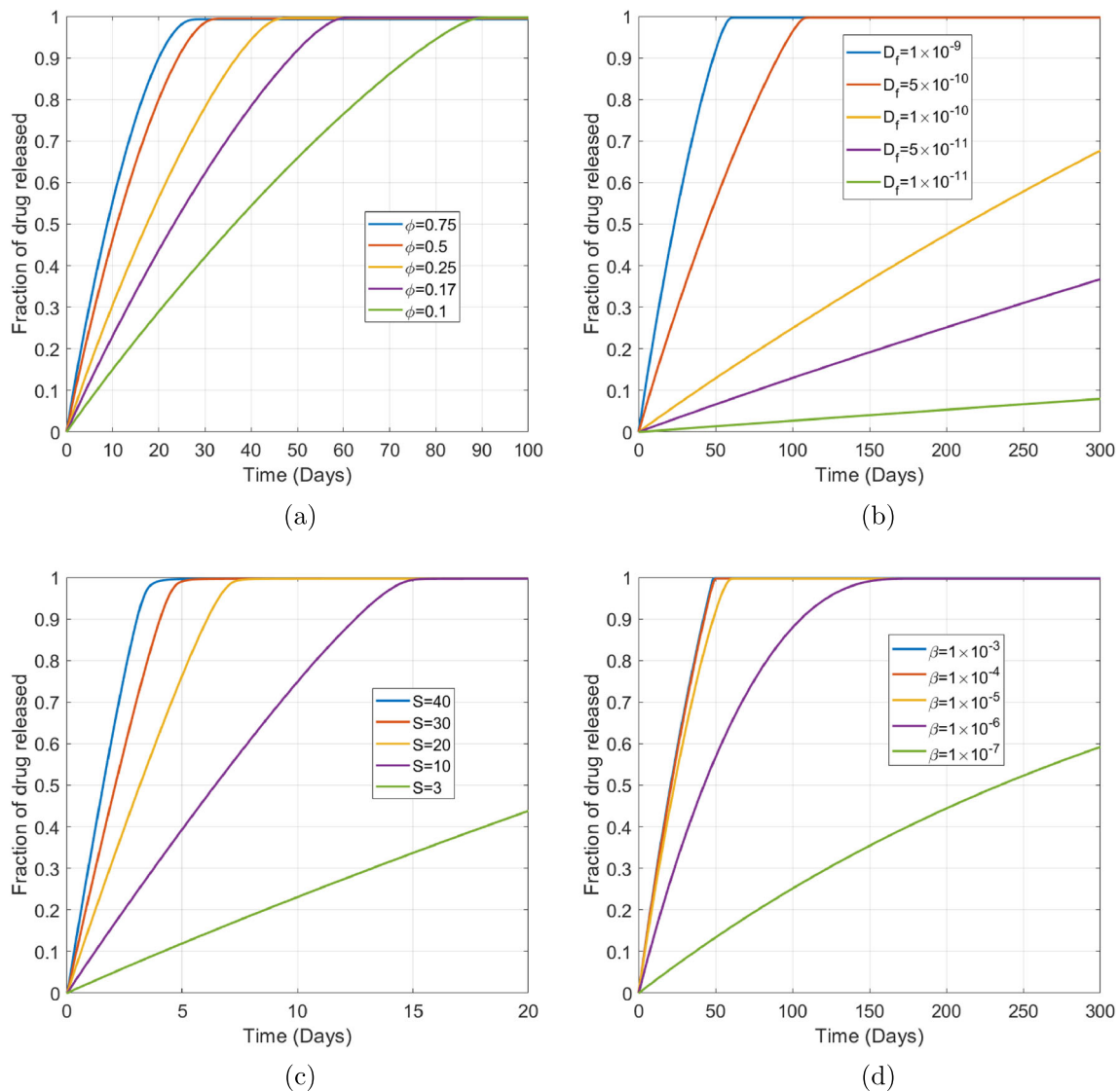
Fig. 13 Plots showing the effect of varying the following porous pin model parameters (a) porosity of the porous wall \phi , (b) free drug diffusion coefficient D_f , (c) drug solubility S and (d) drug dissolution rate \beta . The remaining parameters are baseline parameters as stated in Table 2. The fraction of drug released in all cases was calculated using M_{rel}(t) = \int_{L_d+L_p}^{L_d+L_p+L_m} c_m r dr / b_0 \int_0^{L_d} r dr .
