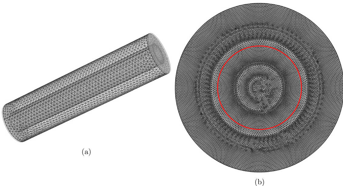
Fig. 8 (a) FEM mesh generated for the 3D porous pin geometry. Mesh consists of 136,059 domain elements, 11,316 boundary elements, and 664 edge elements. (b) FEM mesh generated for the 2D porous pin geometry. Mesh consists of 24,930 domain elements and 472 boundary elements. The red circle indicates the interface between the inner drug core and the porous wall of the geometry.
