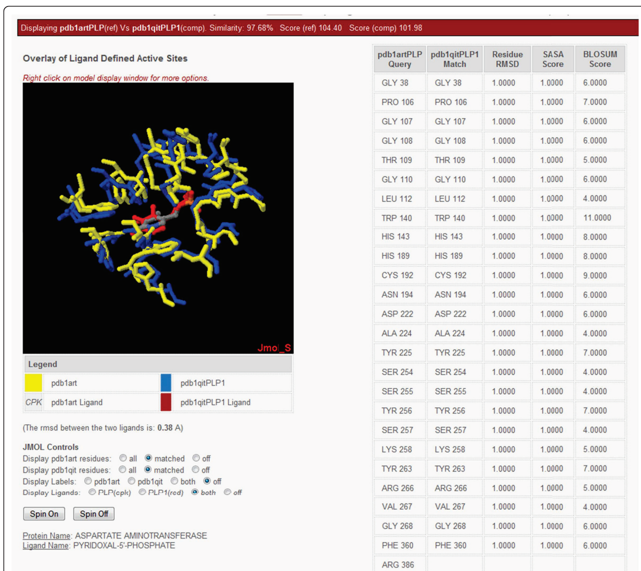
Figure 5 A CPASS alignment summary page is shown that provides a detailed description of the specific ligand-binding site alignment. An interactive Jmol [26] representation of the two aligned ligand defined active sites determined by CPASS is displayed. The RMSD between the two ligands, the protein name and ligand name for the comparison ligand-defined binding site are also provided. The associated table identifies the aligned residues and the per residue \Delta RMSD_{ij} and \Delta SASA_{ij} penalties, and the resulting weighted per residue BLOSUM62 score.
