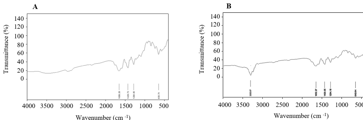
Fig. 4. The structural analysis results of (A) PLGA and (B) OMP-PLGA by FTIR analysis. OMP-PLGA, Outer membrane proteins-poly (lactic-co-glycolic acid).
