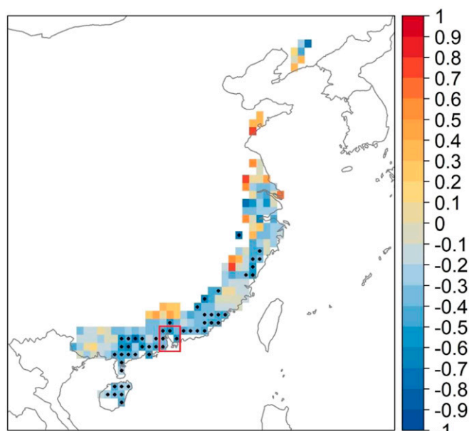
Fig. 2. Spatial pattern of correlation coefficients of translation speeds and local rainfall totals of individual TCs over the coastal areas of China. Only TCs with rainfall intensity (mm/d) \geq 30 mm/d and areas that have at least four TCs with rainfall intensity \geq 30 mm/d are considered. Stippled regions represent areas with Spearman correlation coefficients significant at the 95% level. The red box indicates the location of the Pearl River Delta.
