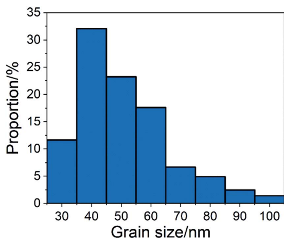
Fig. 2 Grain size distribution of CCNPs after 75 minutes of reaction after adding glucose.
