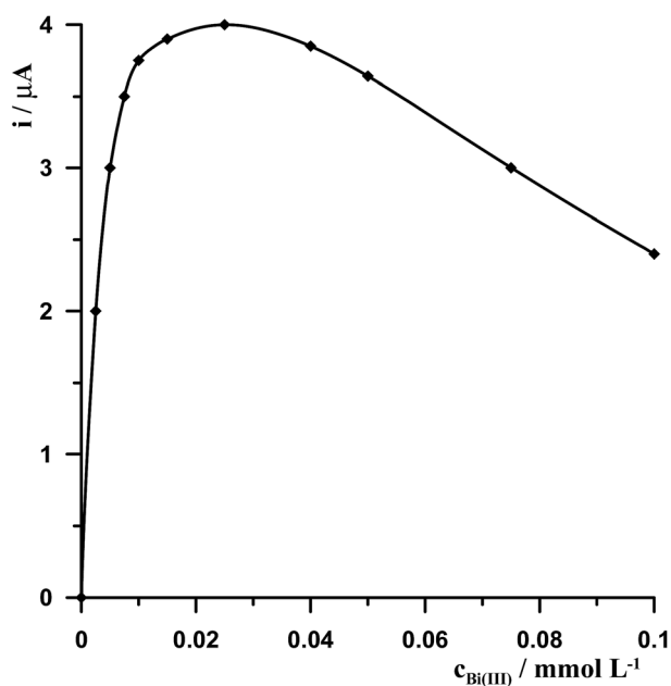
Fig. 1 The influence of \text{Bi(III)} concentration on 5 \times 10^{-8} mol \text{L}^{-1} \text{Ge(IV)} voltammetric signal. Concentrations of 5 \times 10^{-4} mol \text{L}^{-1} chloranilic acid and 0.1 mol \text{L}^{-1} \text{CH}_3\text{COOH} .
