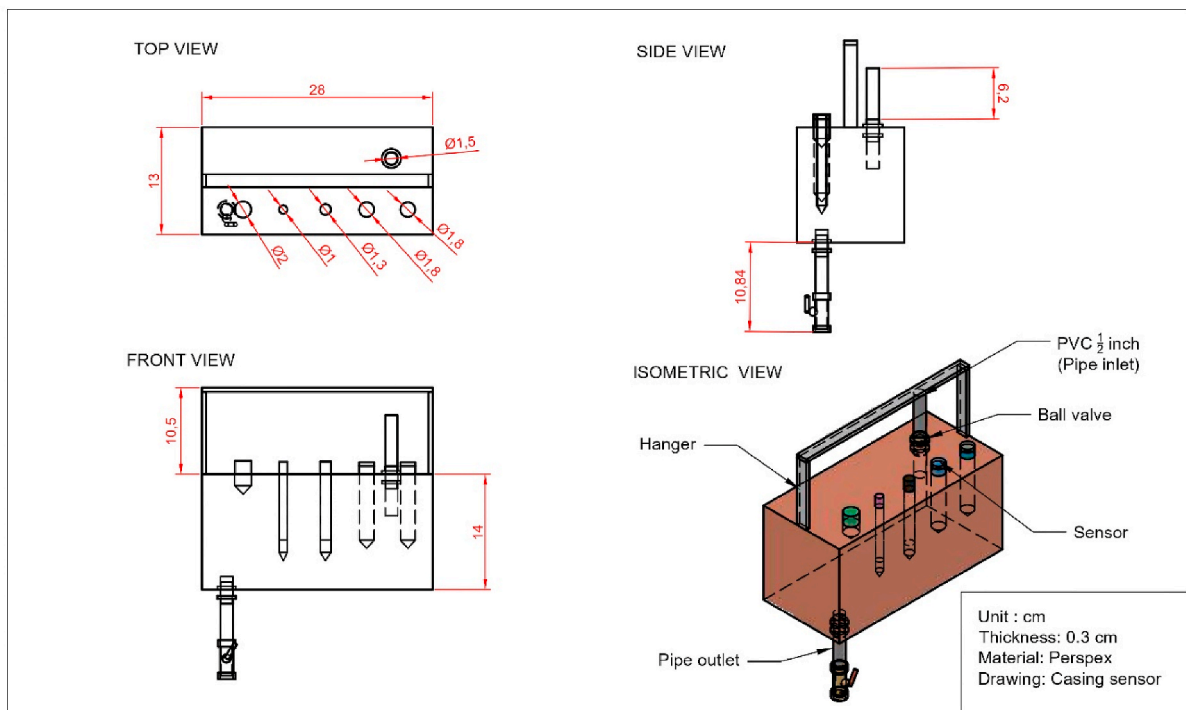
Fig. 15. Sketch of casing sensor using AutoCAD 3D.
