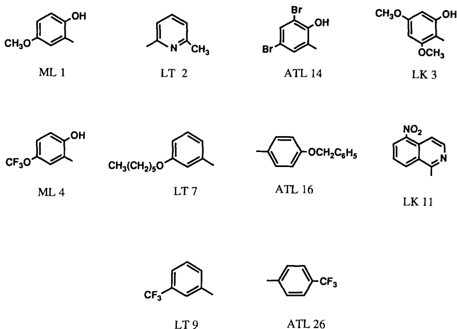
Fig. 1. Structures of the Schiff bases of 1-amino-3-hydroxyguanidine tosylate of the type \text{R-NNH}(\text{C}=\text{NH})\text{NHOH} \cdot \text{HSO}_3\text{C}_6\text{H}_4\text{CH}_3 . The R groups substituted in the 1-position are as follows: compound ML1 2-hydroxy-5-methoxybenzylidene; compound ML4 2-hydroxy-5-trifluoromethoxybenzylidene; compound LT2 (6-methyl-2-pyridyl)-methylene; compound LT7 3-(hexyloxy)benzylidene; compound LT9 3-trifluoro-toluidene; compound ATL14 3,5-dibromo-2-hydroxybenzylidene; compound ATL16 4-benzoyloxybenzylidene; compound ATL26 4-fluoromethoxybenzylidene; compound LK3 2-hydroxy-4, 6-dimethoxybenzylidene; compound LK11 (5-nitroisoquinol-1-yl)-methylene.
