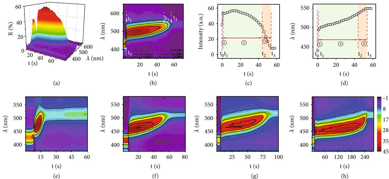
FIGURE 3: Dynamic tracking of solvents diffusion by DRS. (a, b) The dynamic reflection spectrum of solvent diffusion process in the form of a 3D surface map (a) and a contour map (b). (c, d) The intensity (c) and wavelength (d) signals extracted from the contour map. (e–h) DRS patterns resulting from solvent diffusion in PC films that were aged for 1 min (e), 5 min (f), 10 min (g), and 60 min (h) at 70°C.
