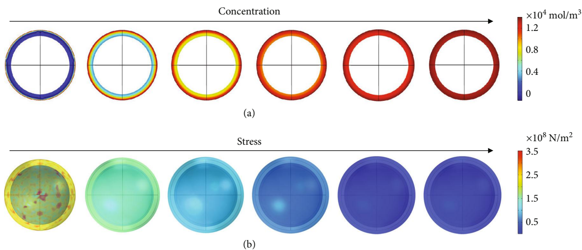
FIGURE 4: Simulation of DMSO diffusion process. Simulation of (a) solvent concentration and (b) shell deformation and stress change during the diffusion of DMSO in an RF shell.
