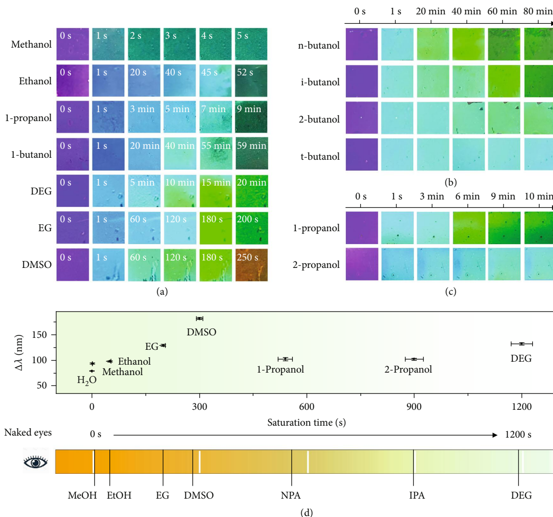
FIGURE 6: Colorimetric sensing of various solvents. (a) Digital photos of PC films infiltrated by methanol, ethanol, 1-propanol, 1-butanol, DEG, EG, and DMSO. (b, c) Digital photos of PC films infiltrated by butanol isomers (b) and propanol isomers (c). (d) Plot showing the wavelength shift vs. the saturated diffusion time for different solvents (upper panel, obtained from DRS) and the saturated diffusion time of solvents observed by naked eyes (bottom panel).
