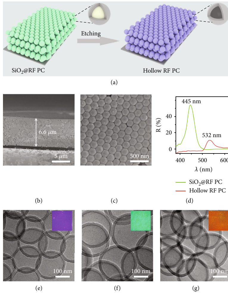
FIGURE 1: Fabrication of hollow RF sphere photonic crystals. (a) Scheme illustrating the fabrication process of photonic crystals consisting of hollow RF spheres. (b, c) SEM images of PC film of hollow RF spheres: cross-section (b) and top-view (c). (d) Reflectance spectra of PC films before and after removing silica. (e–g) TEM images of hollow RF spheres with diameters of 210 nm (e), 245 nm (f), and 275 nm (g). The insets are dark-field optical microscopy images of the corresponding PCs.
