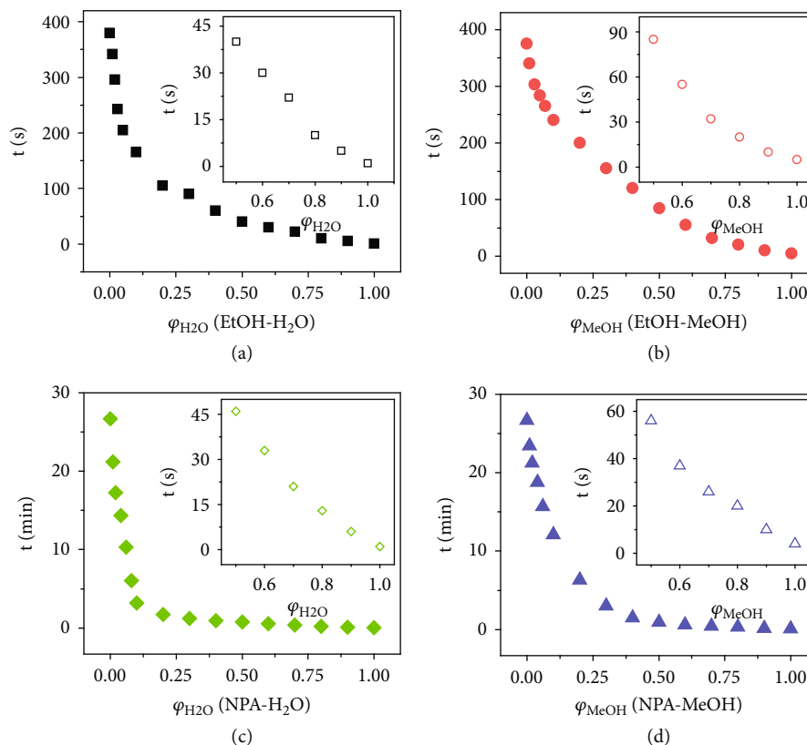
FIGURE 7: Quantitative determination of component concentration. The saturated diffusion time of various solvent mixtures in PC films: (a) ethanol and water, (b) ethanol and methanol, (c) 1-propanol and water, and (d) 1-propanol and methanol. The insets are the close-ups of the plots for the volume fraction between 0.5 and 1. The PC films were predried for 24 h at 70°C.
