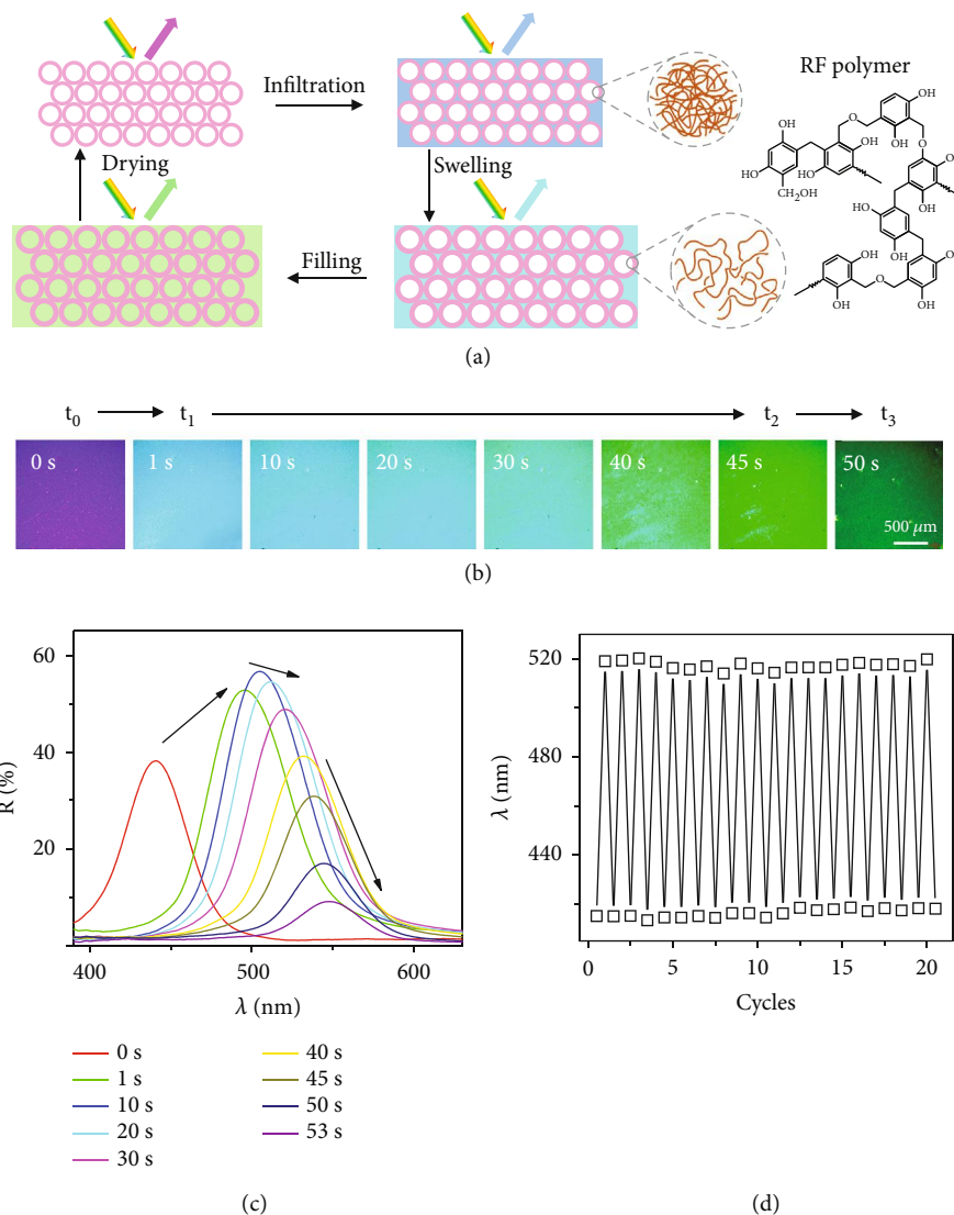
FIGURE 2: Typical three-step diffusion process of solvents. (a) Scheme illustrating the three-step diffusion of solvents in the hollow-sphere PCs. (b, c) Dark-field optical microscopy images (b) and corresponding reflectance spectra (c) during ethanol diffusion in the PC film. (d) Changes of reflection wavelength in response to repeated infiltration with ethanol and then drying for 20 cycles.
