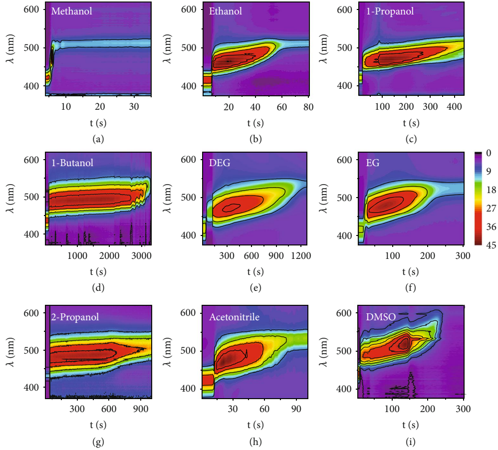
FIGURE 5: DRS patterns of various polar solvents. DRS patterns resulting from the diffusion of various solvents in PC films: (a) methanol, (b) ethanol, (c) 1-propanol, (d) 1-butanol, (e) DEG, (f) EG, (g) 2-propanol, (h) acetonitrile, and (i) DMSO.
