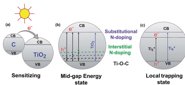
Fig. 4 Reduction of the TiO 2 -BSP band gap energy via sensitizing (a), forming a mid-gap energy state (b) and forming a local trapping state (c).
