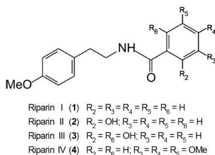
Figure 1. Chemical structure of riparins I, II, III and IV.
