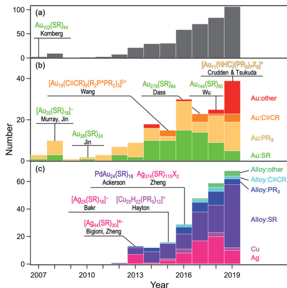
Fig. 1 Annual numbers of crystals data of (a) coinage-metal MPCs, (b) Au MPCs, and (c) Ag/Cu/ally MPCs deposited in the Cambridge Crystallographic Data Centre since 2007, with selected benchmark studies.
