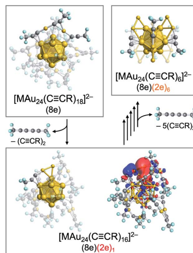
Fig. 12 Scheme of the formation of superatomic assemblies via CID of 1,3-diyne from [\text{MAu}_{24}(\text{C}\equiv\text{CR})_{18}]^{2-} . Color code: yellow = Au; gray = C; light blue = F.
