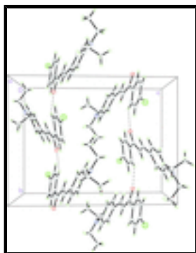
Fig. 2. The crystal packing of the title compound view along the a -axis, showing ribbons running along the b axis. Hydrogen bonds are shown as dashed lines.
