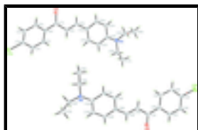
Fig. 1. Two independent molecules of the title compound, with 50% probability displacement ellipsoids and the atom-numbering scheme.
