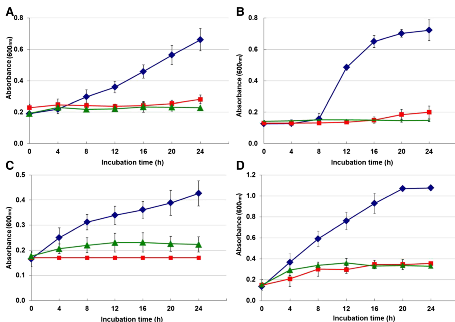
Figure 2 Growth curves of different bacterial strains exposed to Vespa orientalis crude venom during 24 hours. (A) Staphylococcus aureus with 64 µg/mL, (B) Bacillus subtilis with 8 µg/mL, (C) Escherichia coli with 64 µg/mL and (D) Klebsiella pneumonia with 128 µg/mL compared with tetracycline with 16 µg/mL at 37°C. (blue diamond symbol): Control, (red square symbol): tetracyclin, (green triangle symbol): wasp crude venom.
