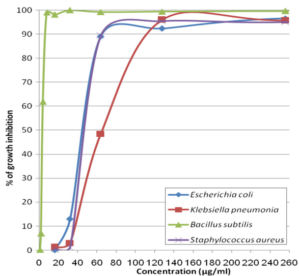
Figure 3 Inhibitory effect of various concentrations of Vespa orientalis crude venom on the growth of different bacterial strains.
