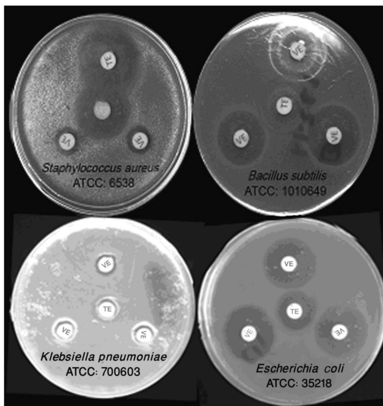
Figure 1 Inhibitory effect of Vespa orientalis (VE: venom extract, 30 µg/disc) on the growth of different bacterial strains compared with tetracycline (TE: tetracycline, 30 µg/disc).
