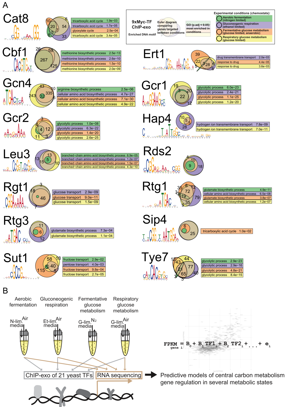
Figure 1. (A) Genome-wide TF binding characterization for multiple conditions of 15 TFs first described in this study. The most enriched DNA sequence (defined by MEME) is indicated under the TF name. The euler diagrams indicate the number of genes targeted between the experimental conditions and how the conditions overlap. Numbers are shown for all overlaps with more than two genes. For each condition, the top significant (if there is any with P_{adj} < 0.05 ) GO category for the genes targeted that condition is shown in the same color color of the condition in the euler diagram. (B) A summary of our experimental approach.
