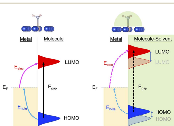
Scheme 1 Illustration of the effect of solvent on the excitation energy. The presence of solvent shifts the energy levels of the molecular frontier orbitals (HOMO and LUMO) with respect to the metal Fermi level ( E_F ). An \text{NH}_3 molecule is used in the atomic structures to illustrate the concept.
