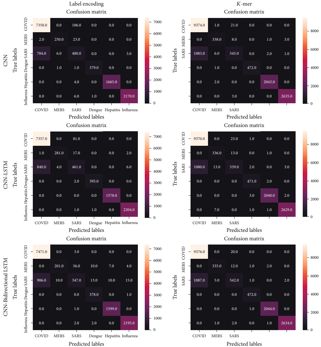
FIGURE 9: Confusion matrix of Label encoding and K -mer encoding for DNA sequence classification.
