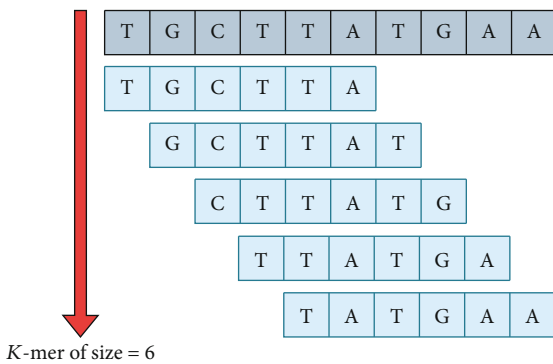
FIGURE 5: Sequence data encoding using the K -mer technique.
