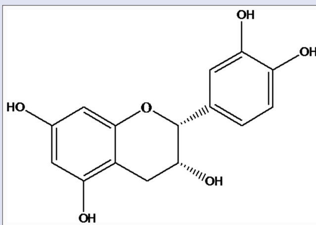
Figure 1: The chemical structure of epicatechin
