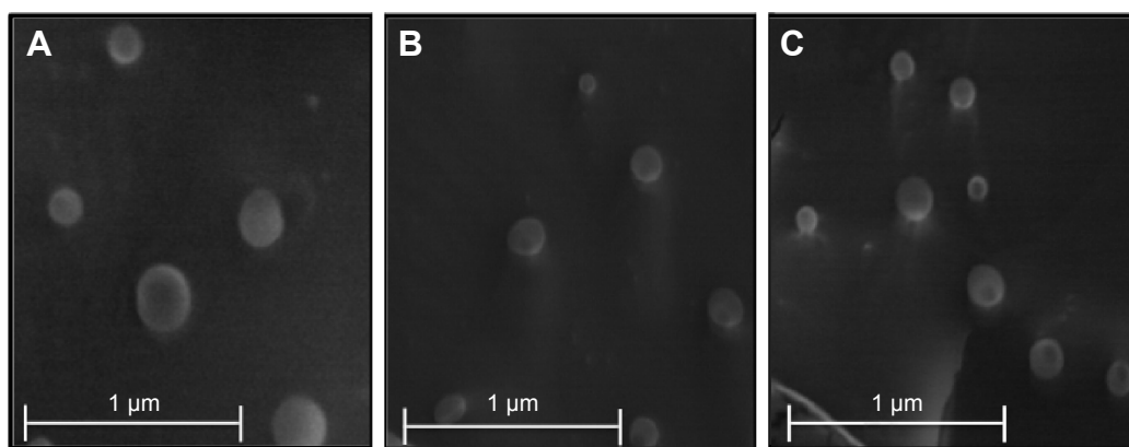
Figure 1 Cryo-SEM images of (A) NLC, (B) M-NLC, and (C) M-NLC-RFB at 20,000 \times magnification. Abbreviations: NLC, nanostructured lipid carrier; M, mannose; RFB, rifabutin; SEM, scanning electron microscopy.
