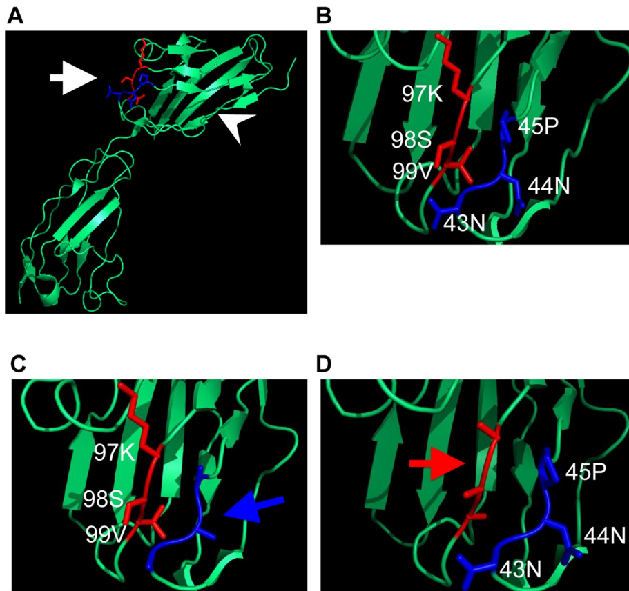
FIGURE 2: JAM-A mutants have alterations in the putative trans -dimerization interface. (A) JAM-A cis -dimerization occurs by ionic interactions between residues located on the C, C', F, G \beta -sheet of the D1 domain (arrowhead), whereas trans -dimerization is predicted to occur on the opposite face of D1 (arrow). (B) The predicted site for trans -dimerization involves two motifs composed of residues N43–P45 and K97–V99, which combine to form a groove. The NNP mutant contains alanine substitutions of amino acids N43–P45 (C, blue arrow), and the KSV mutant contains alanine substitutions of amino acids K97–V99 (D, red arrow).
