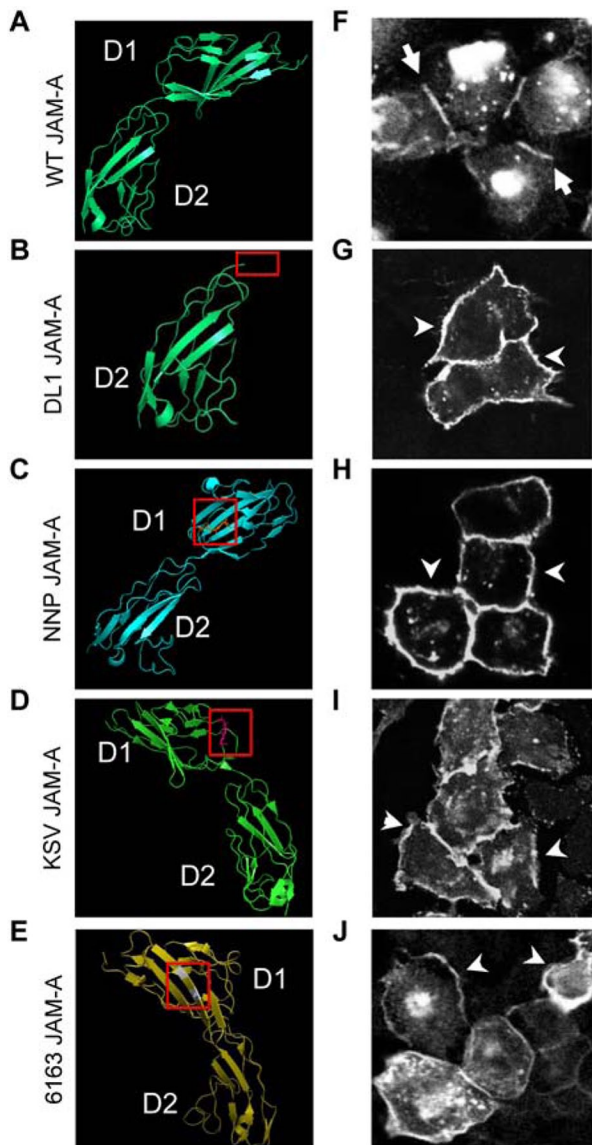
FIGURE 3: Subcellular localization of JAM-A mutants. (A–E) JAM-A cis - and predicted trans -dimer mutants were engineered using site-directed mutagenesis. (A) WT JAM-A is composed of two extracellular Ig-like domains, the most distal of which (D1) is involved in JAM-A homodimerization. (B) DL1 JAM-A lacks the entire membrane-distal Ig-like domain, with only the membrane proximal domain (D2) remaining. (C) NNP JAM-A has alanine substitutions of amino acids 43N, 44N, and 45P, which are predicted to be involved in
