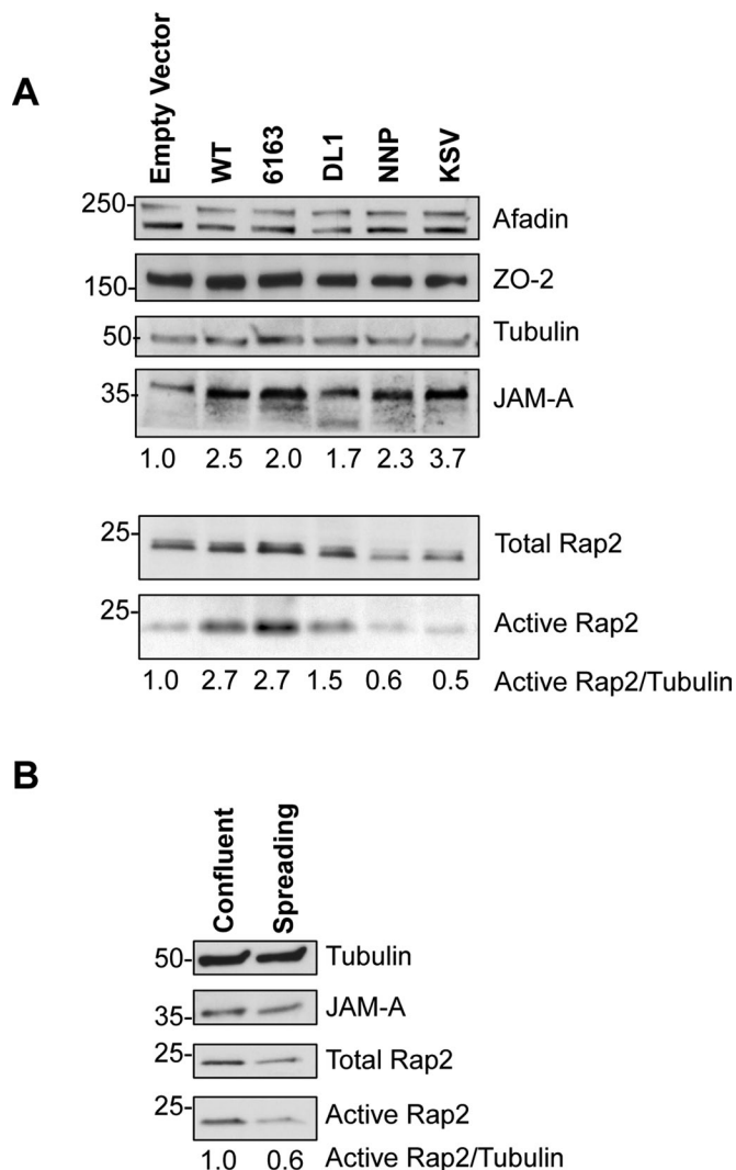
FIGURE 7: JAM-A trans - but not cis -dimerization is required for Rap2 activity. (A) WT and mutant JAM-A were expressed in HEK-293T cells. Cells were assessed for Rap2 activity by Ral-GDS precipitation. (B) Rap2 activity in confluent or spreading human intestinal epithelial cells (SK-CO15) was assessed with Ral-GDS precipitation.
