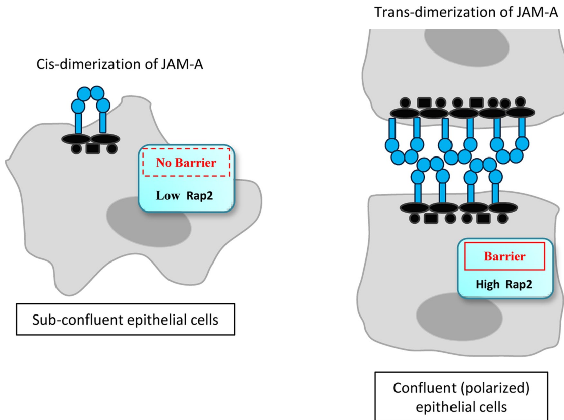
FIGURE 8: JAM-A dimerization in cis may initiate different signaling modalities than that initiated by JAM-A multimerization, which is dependent on trans -dimerization. Left, subconfluent epithelial cells may engage JAM-A cis -homodimers. In the absence of cell–cell contacts (no barrier), the level of active Rap2 is low. Under these conditions, cell migration and spreading are regulated by JAM-A cis -dimerization and increased Rap1. Right, JAM-A trans -dimerization in confluent monolayers of polarized epithelial cells is associated with a tight barrier. Signaling events downstream of JAM-A trans -dimerization lead to the activation of Rap2, which contributes to barrier regulation.
