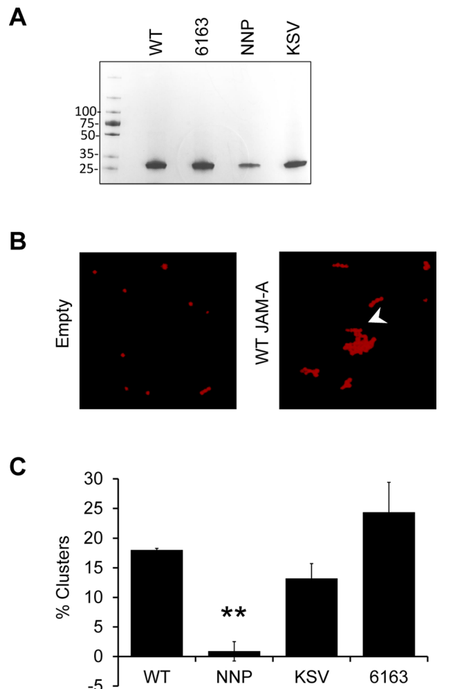
FIGURE 5: JAM-A–conjugated beads cluster as determined by flow cytometry. (A) Bacterially expressed recombinant ectodomains of WT and mutant JAM-A with a C-terminal His tag were purified and analyzed by SDS–PAGE. (B) His-binding 1- \mu m beads conjugated to His-tagged WT JAM-A clustered in solution (arrowhead) compared with unconjugated beads. Bead clustering was quantified by assessing side and forward scatter using flow cytometry, by which frequency of unclustered beads was measured as a function of total beads. Flow cytometry data were pooled, and the frequency of clustering was calculated by subtracting frequency of unclustered beads from 100%. Baseline clustering observed in unconjugated beads (frequency \sim 30\% ) was considered to be background and was subtracted from the final readings observed in experiments using WT, NNP, KSV, and 6163 JAM-A–conjugated beads (C; n > 3 per group, mean \pm SEM. ** p < 0.01 compared with WT).
