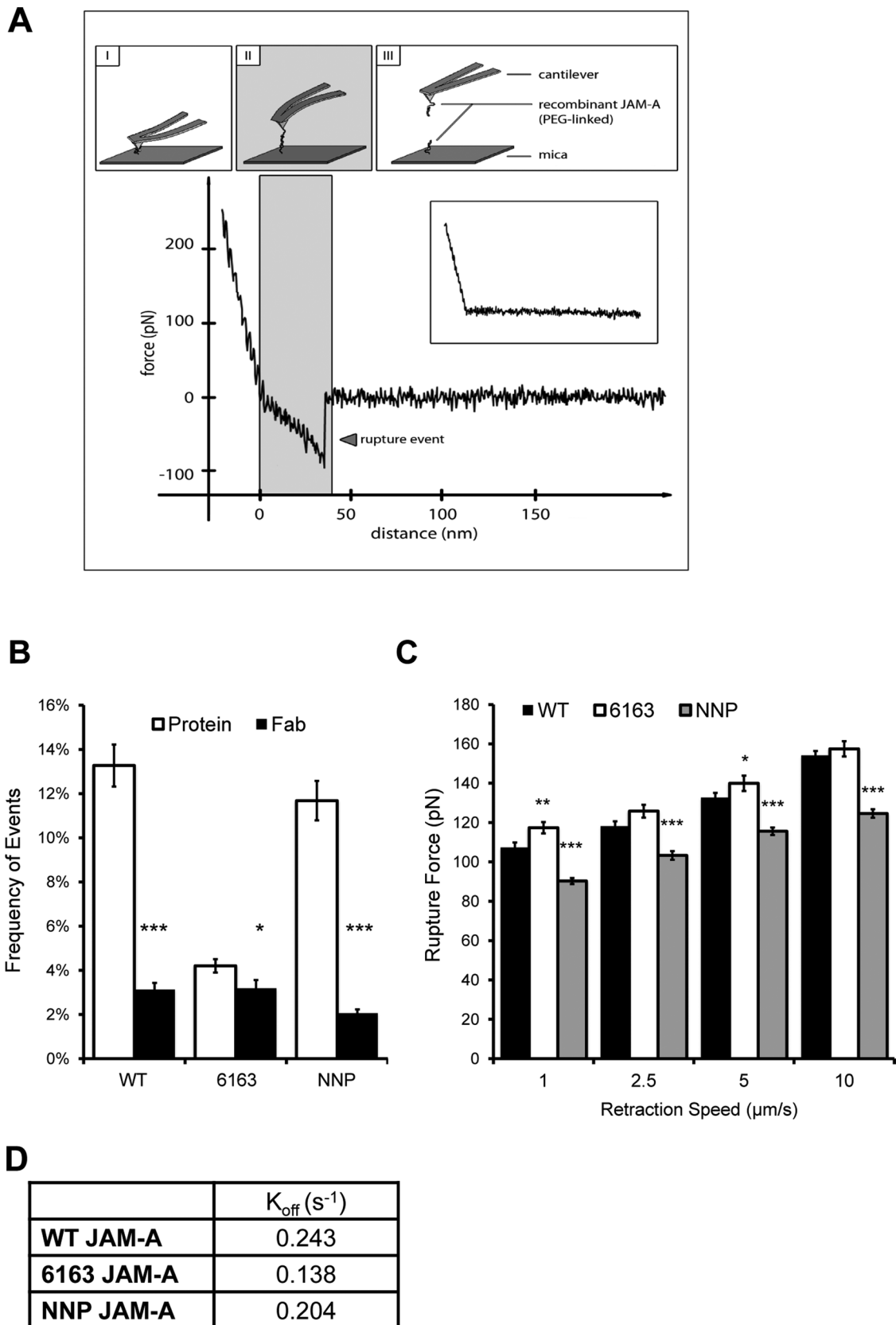
FIGURE 6: Atomic force microscopy reveals that JAM-A can form cis - and trans -dimers. (A) Principle of AFM force spectroscopy. A flexible cantilever (nominal spring constant 0.03 N/m), functionalized with recombinant JAM-A, is lowered onto a mica sheet also coated with the same JAM-A molecules until the cantilever is observed to be bending slightly upward (I). In the event of binding interactions between molecules on the cantilever and mica sheet, as the cantilever is retracted, it bends downward, and the forces are quantified. Forces acting on the cantilever are determined
