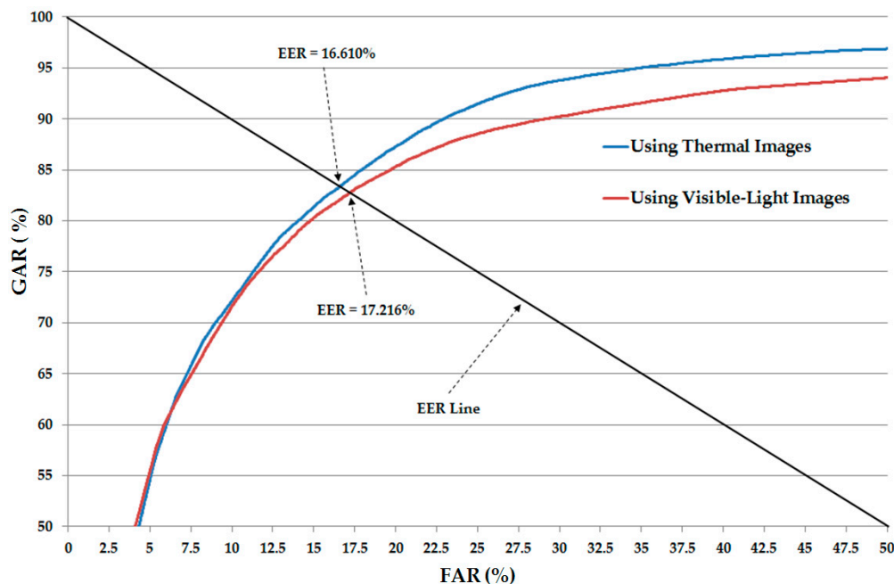
Figure 6. Average ROC curves of recognition systems using single image types with the CNN-based method in Figure 2.
